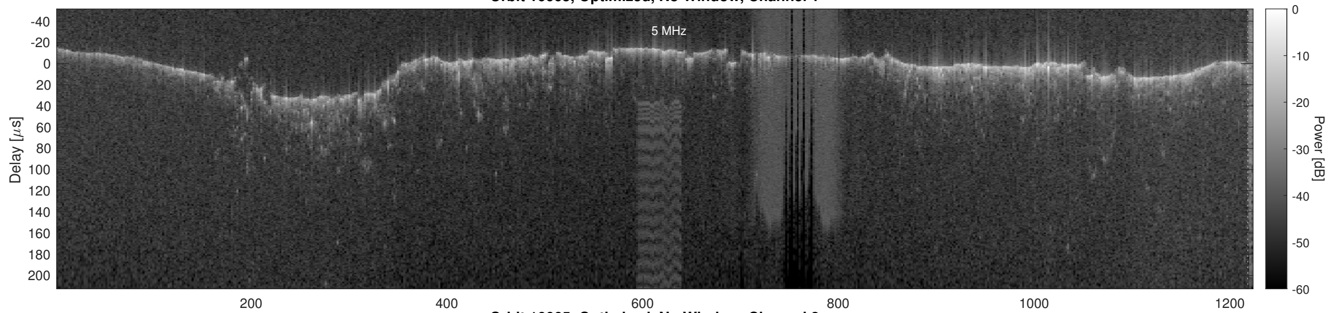
Orbit 16665, Optimized, No Window, Channel 2
