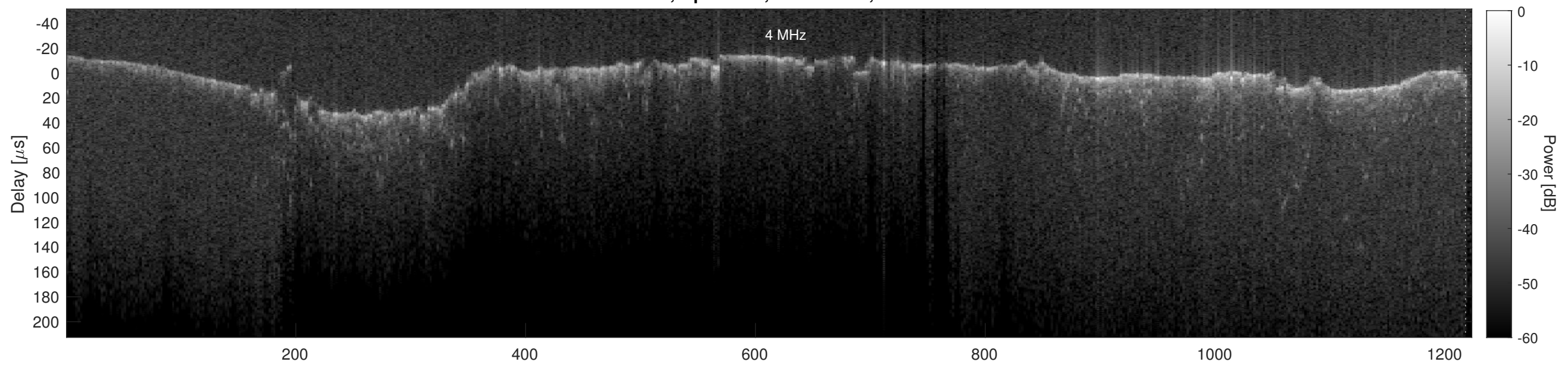
Orbit 16665, Cluttergram
