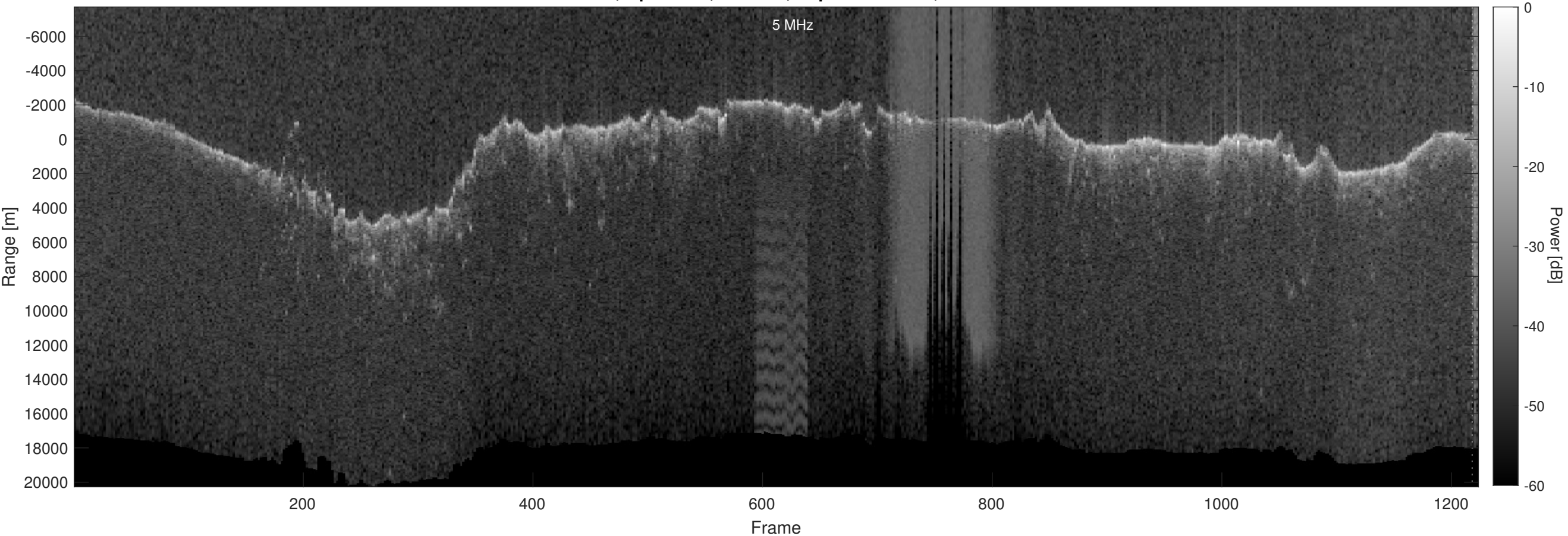
Orbit 16665, Optimized, Window, Depth-Corrected, Channel 2
