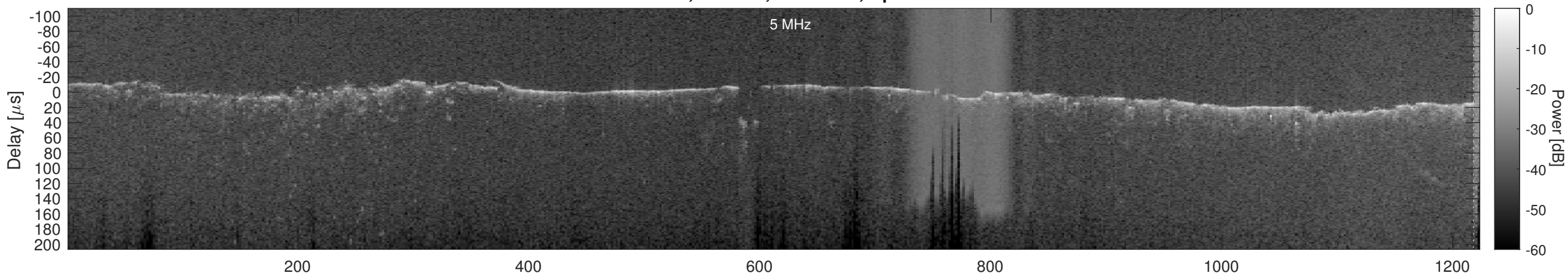
Orbit 16666, Cluttergram
