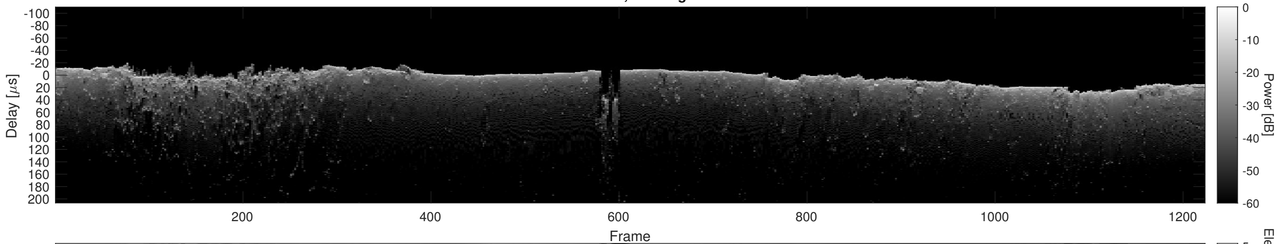
Orbit 16666, Cluttergram
