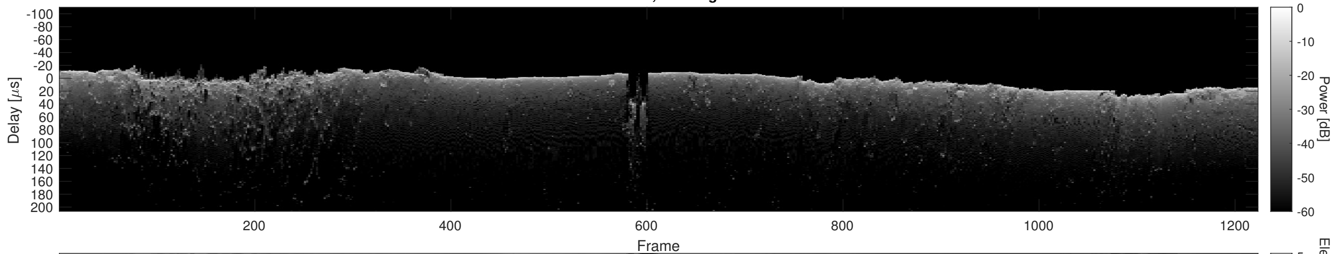
Orbit 16666, Cluttergram
