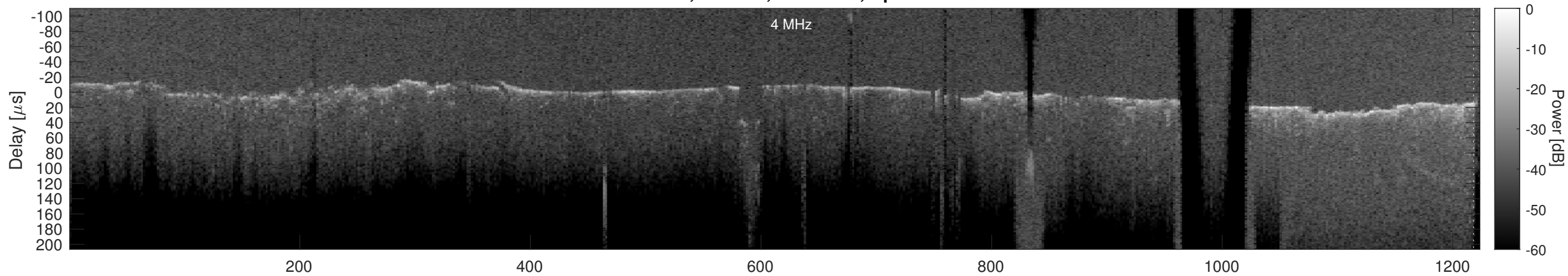
Orbit 16666, Cluttergram
