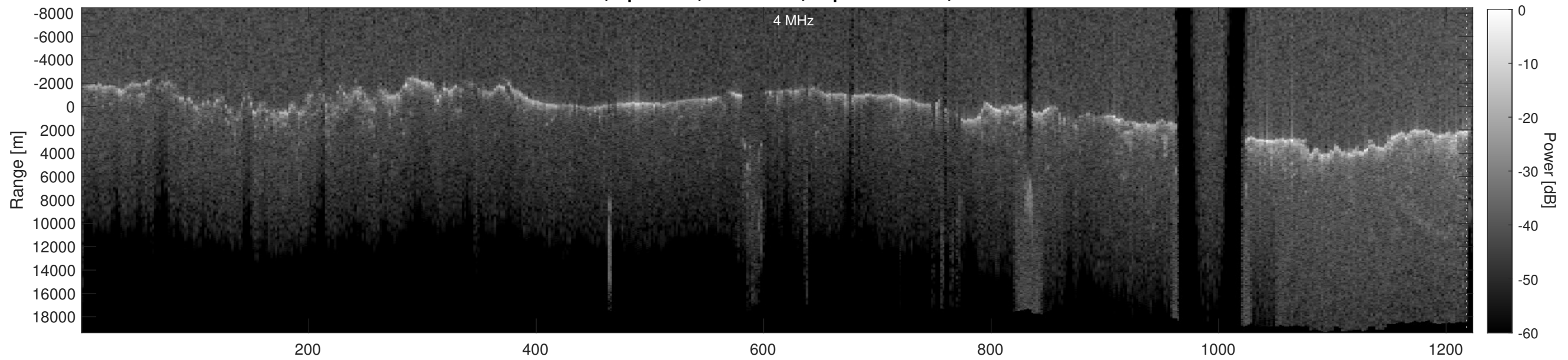
Orbit 16666, Depth-Corrected Cluttergram
