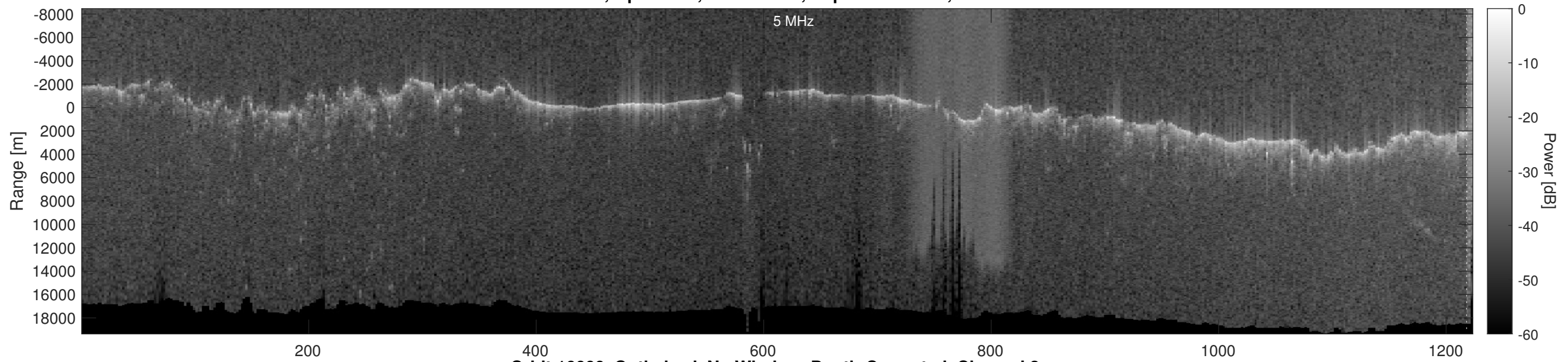
Orbit 16666, Optimized, No Window, Depth-Corrected, Channel 2
