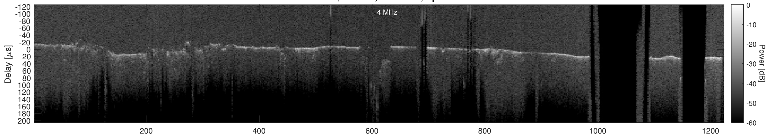
Orbit 16673, Cluttergram
