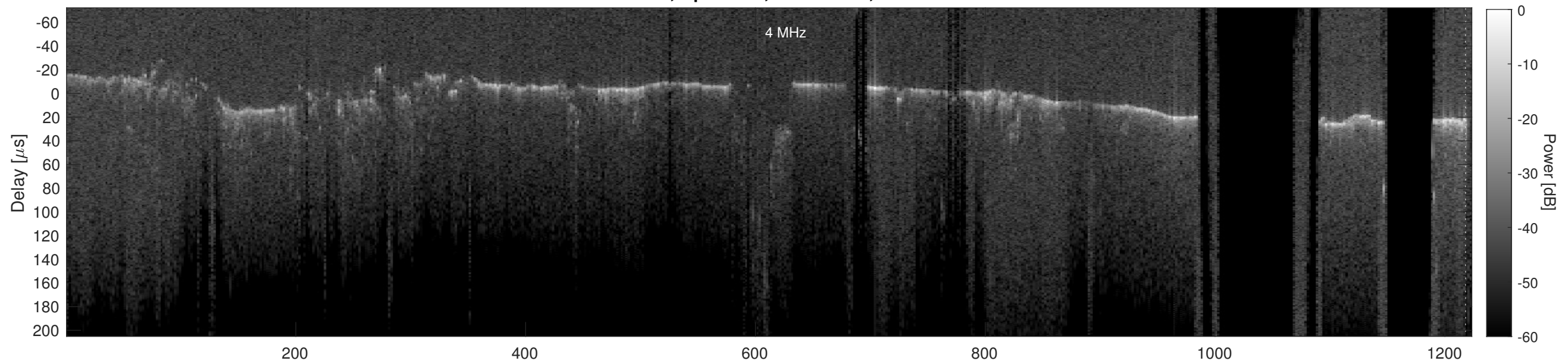
Orbit 16673, Cluttergram
