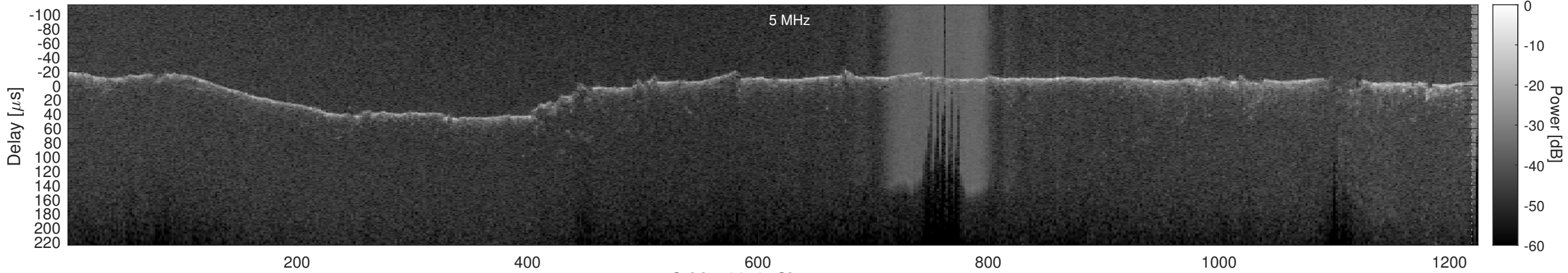
Orbit 16679, Cluttergram
