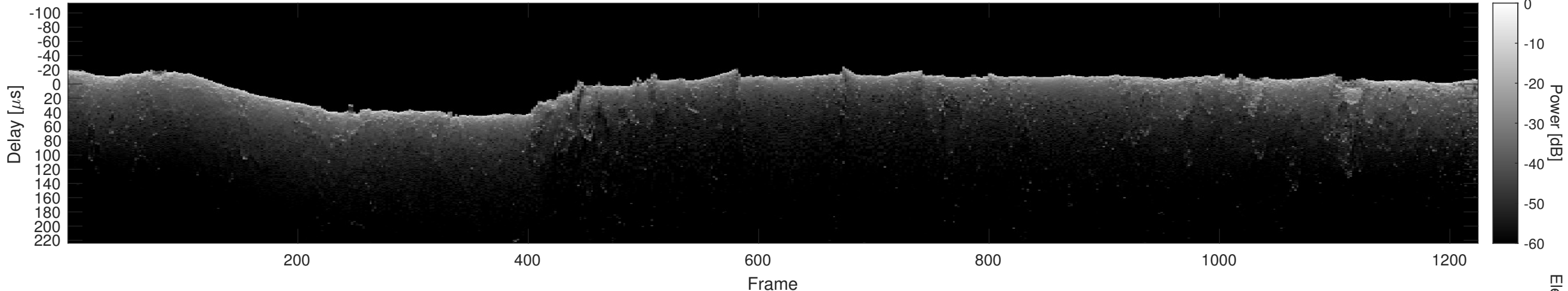
Orbit 16679, Cluttergram
