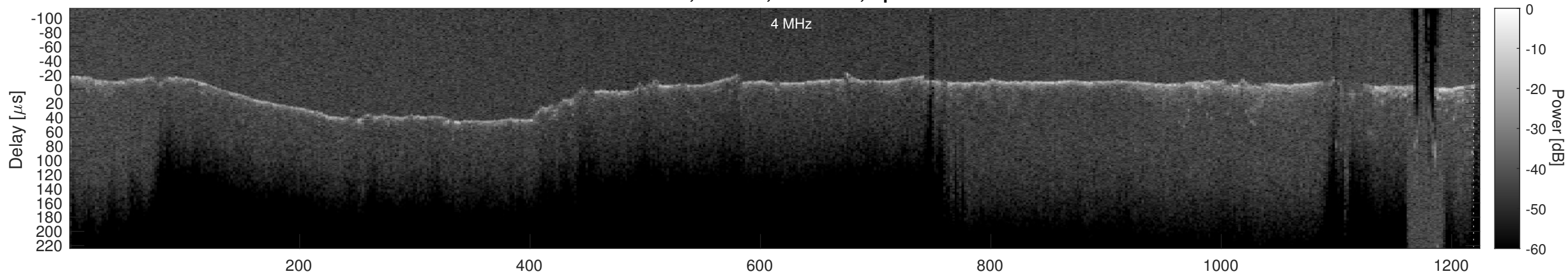
Orbit 16679, Cluttergram
