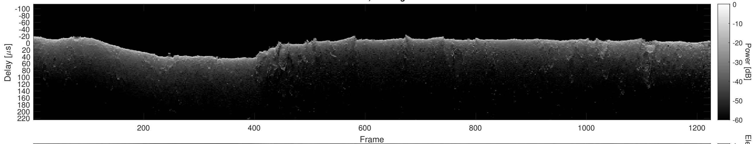
Orbit 16679, Cluttergram
