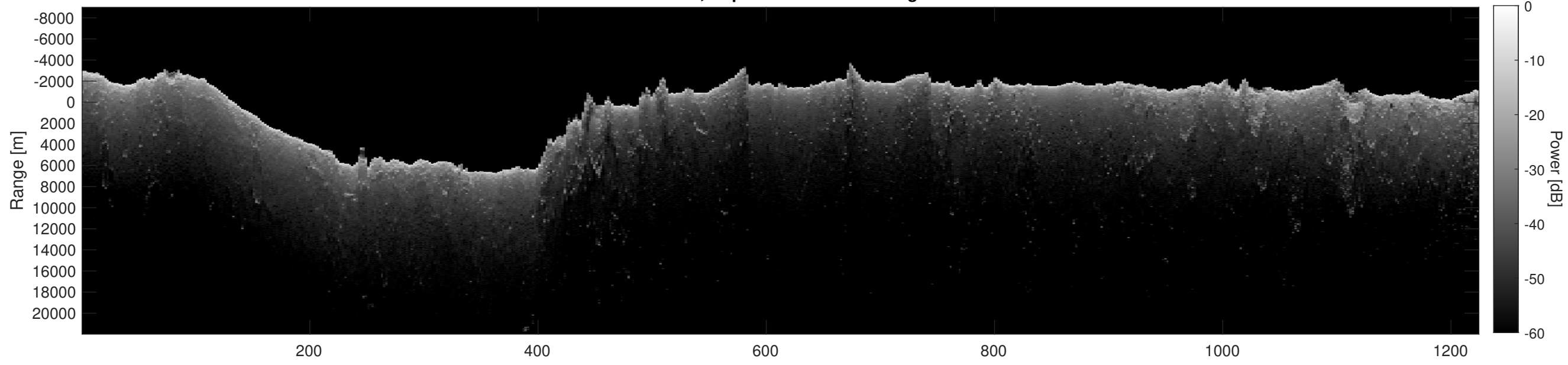
Orbit 16679, Depth-Corrected Cluttergram
