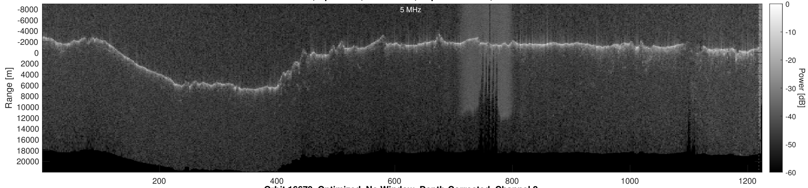
Orbit 16679, Optimized, No Window, Depth-Corrected, Channel 2
