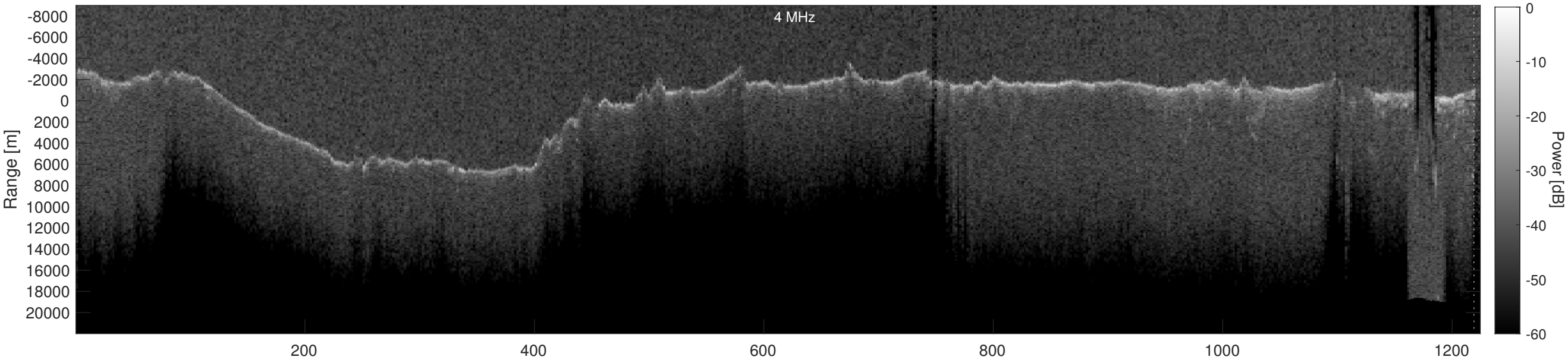
Orbit 16679, Depth-Corrected Cluttergram
