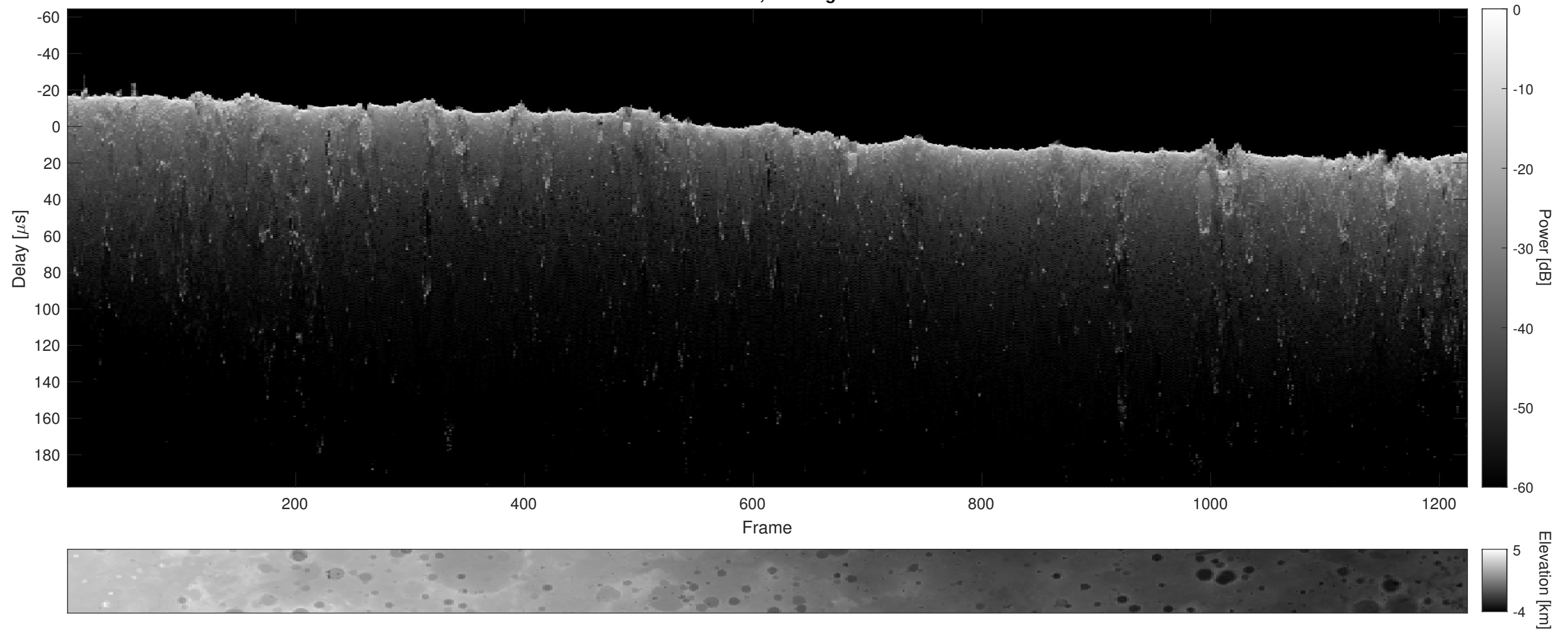
Orbit 16683, Cluttergram
