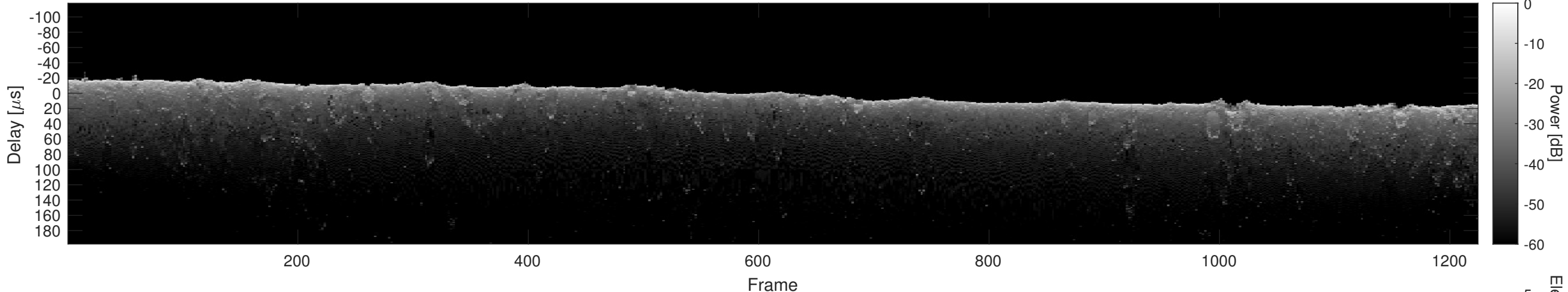
Orbit 16683, Cluttergram
