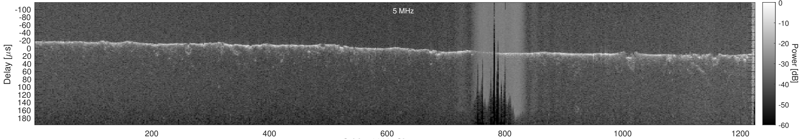
Orbit 16683, Cluttergram
