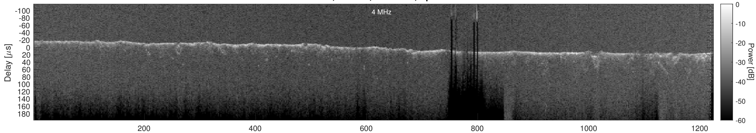
Orbit 16683, Cluttergram
