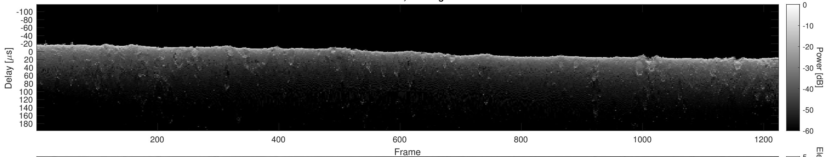
Orbit 16683, Cluttergram
