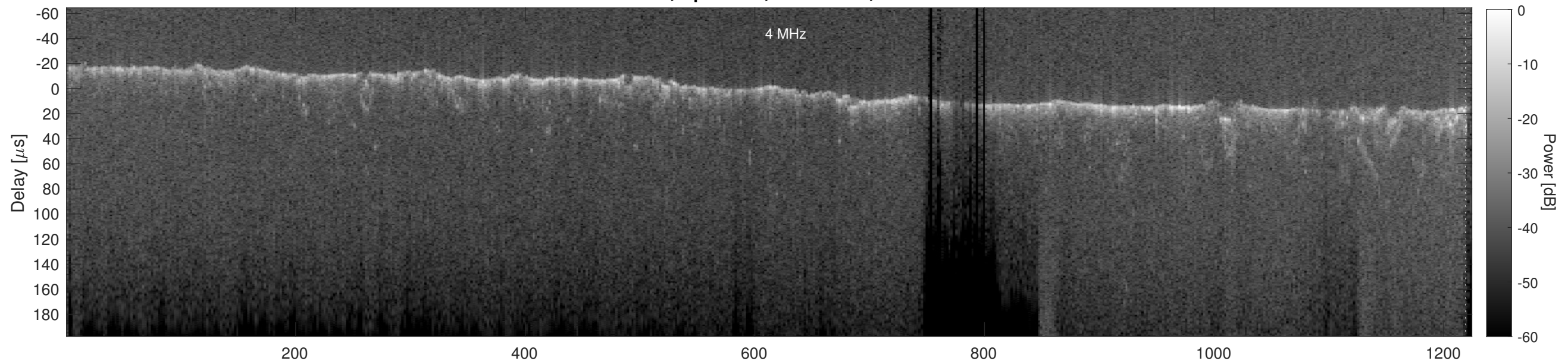
Orbit 16683, Cluttergram
