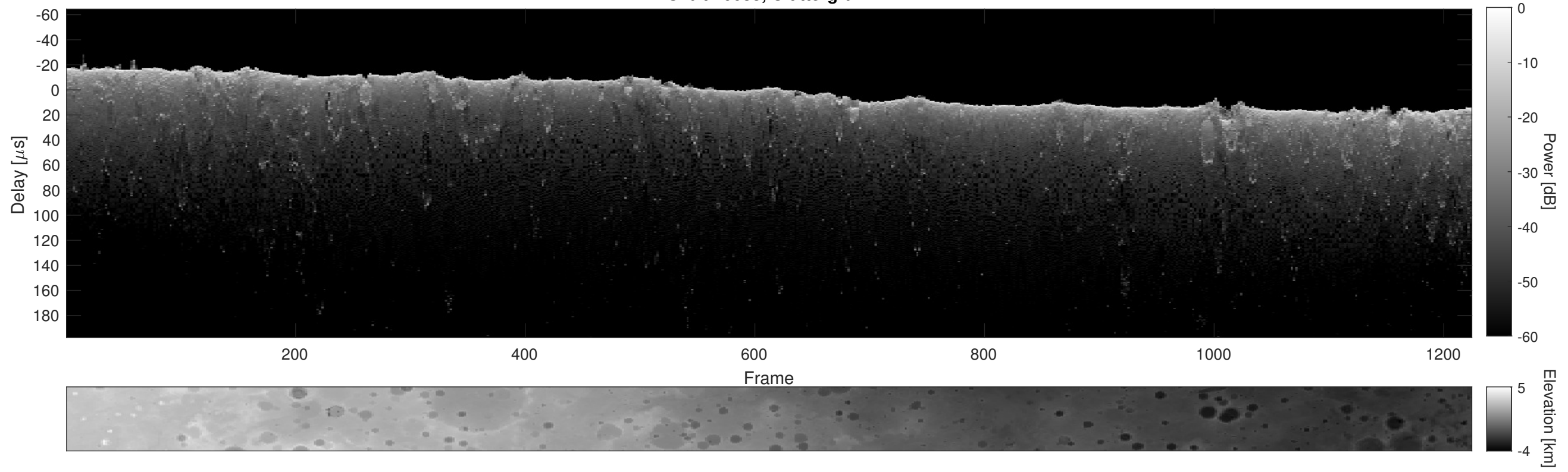
Orbit 16683, Cluttergram
