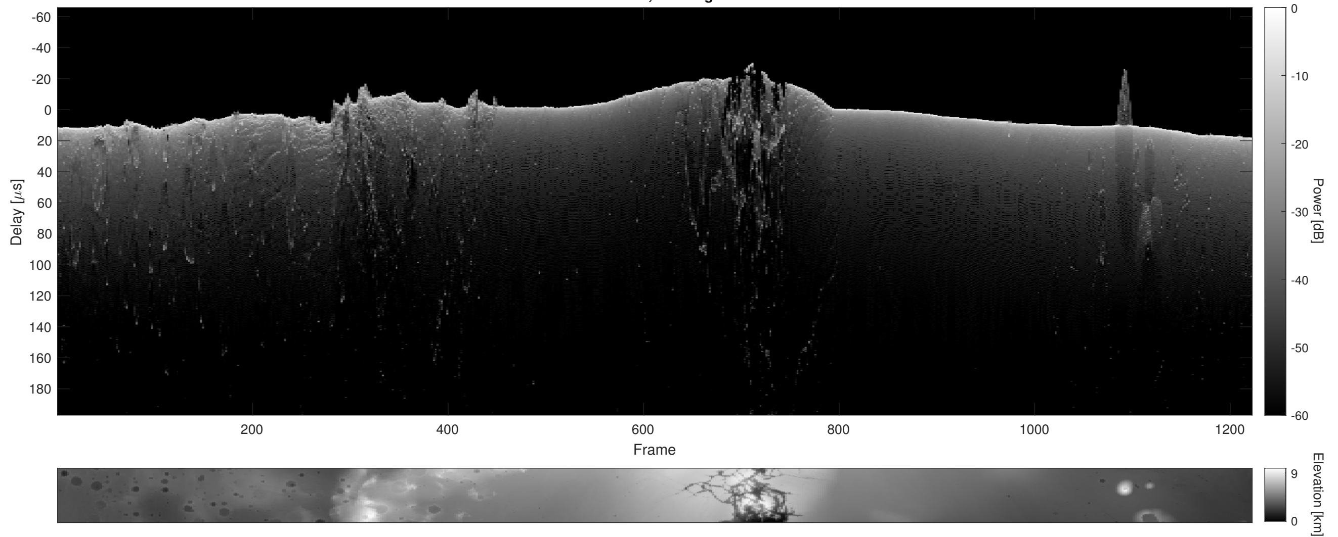
Orbit 16684, Cluttergram
