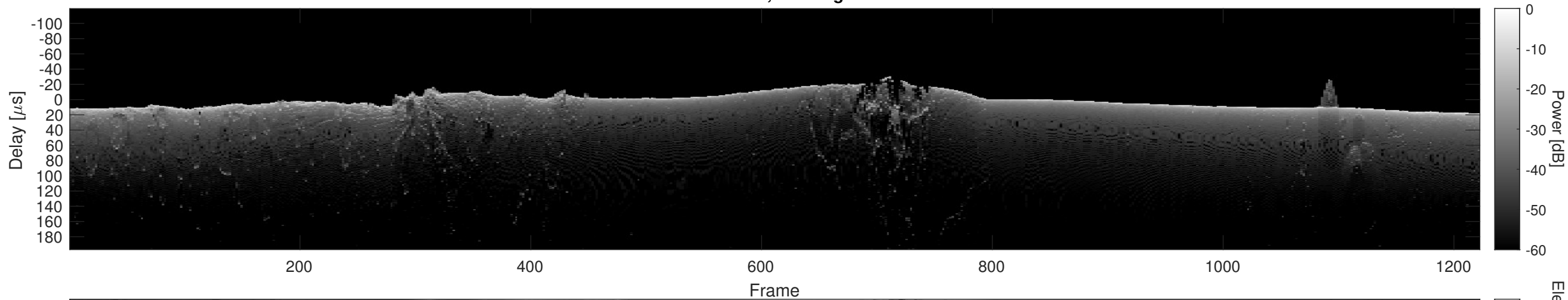
Orbit 16684, Cluttergram
