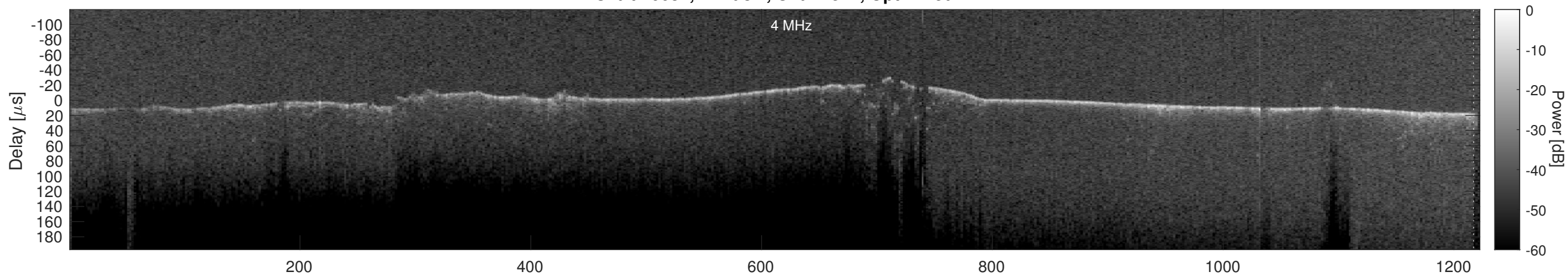
Orbit 16684, Cluttergram
