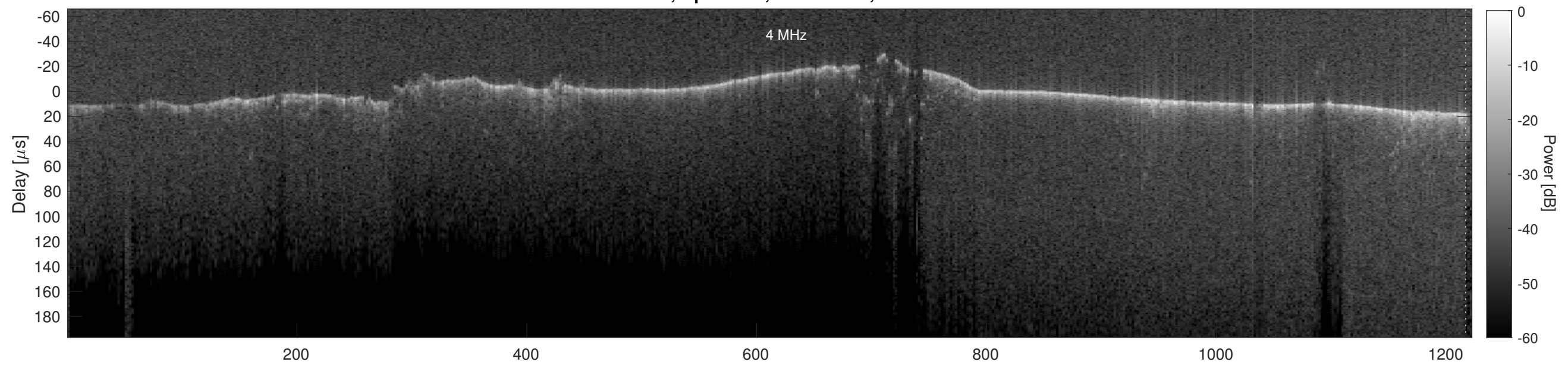
Orbit 16684, Cluttergram
