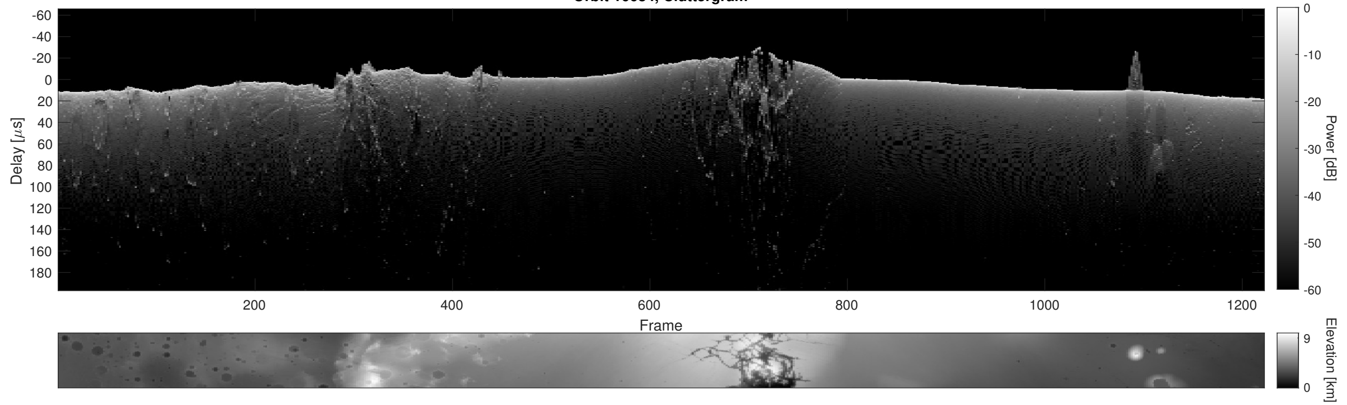
Orbit 16684, Cluttergram
