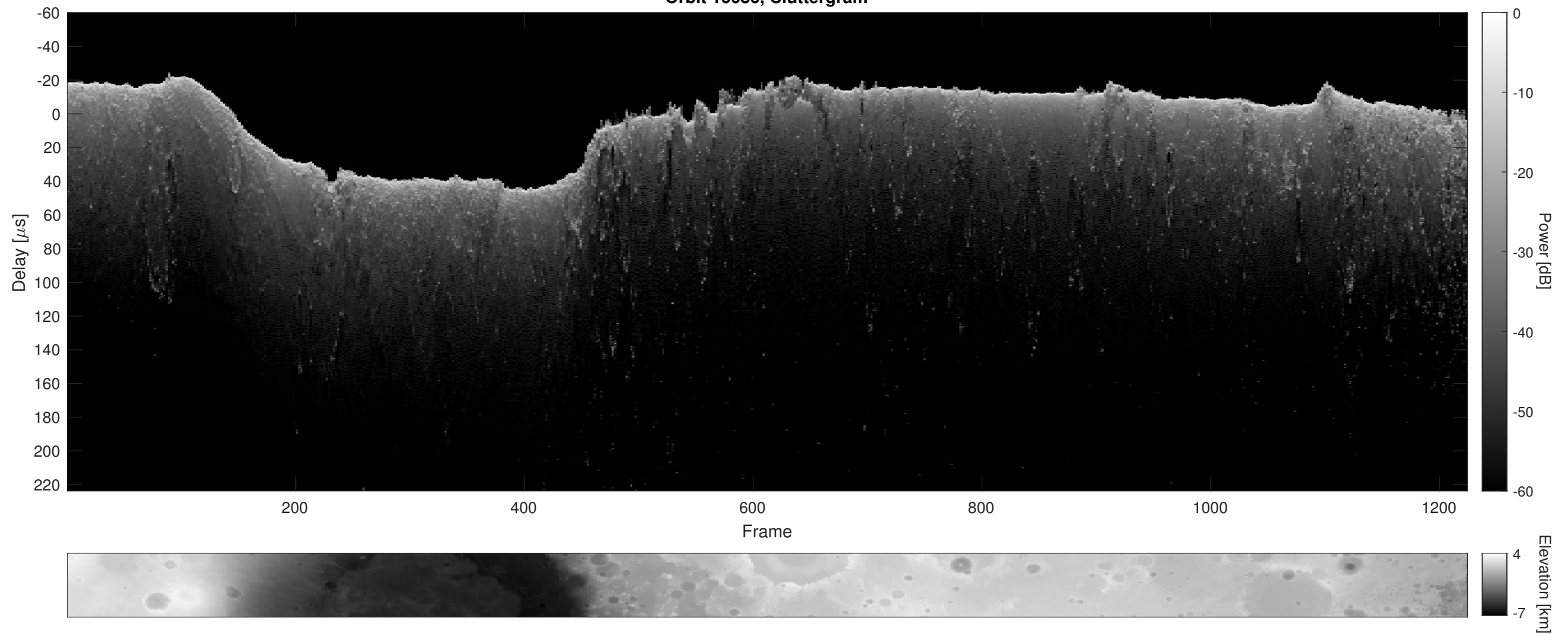
Orbit 16686, Cluttergram
