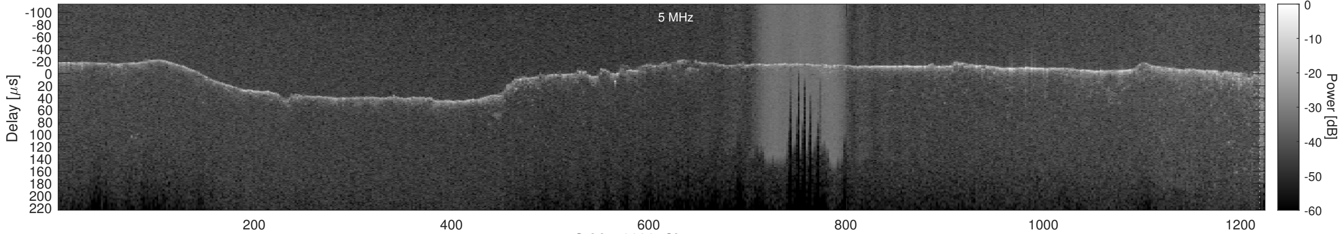
Orbit 16686, Cluttergram
