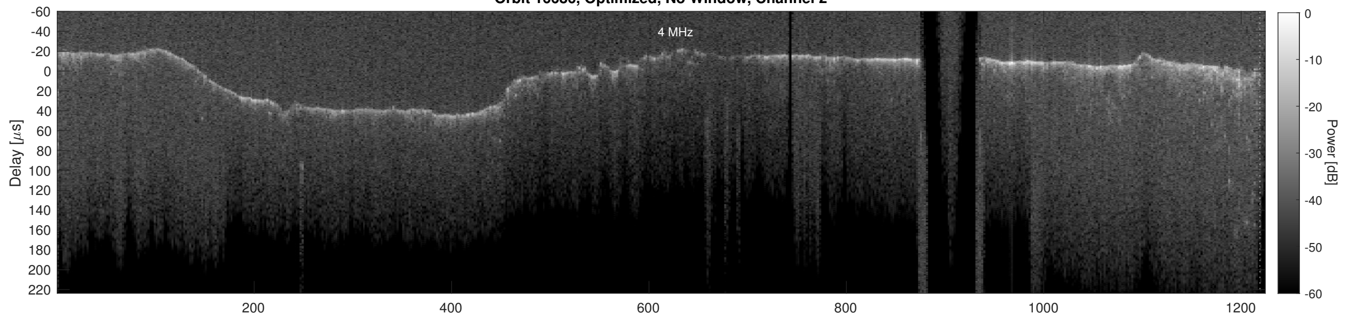
Orbit 16686, Cluttergram
