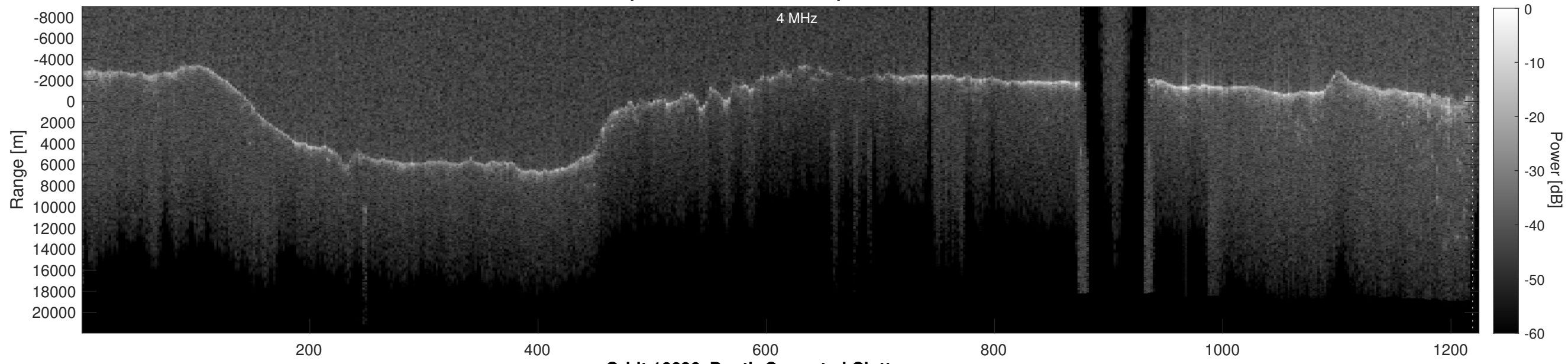
Orbit 16686, Depth-Corrected Cluttergram
