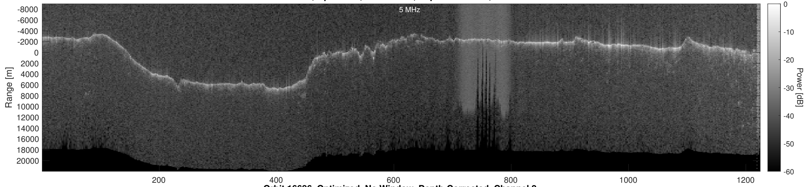
Orbit 16686, Optimized, No Window, Depth-Corrected, Channel 2
