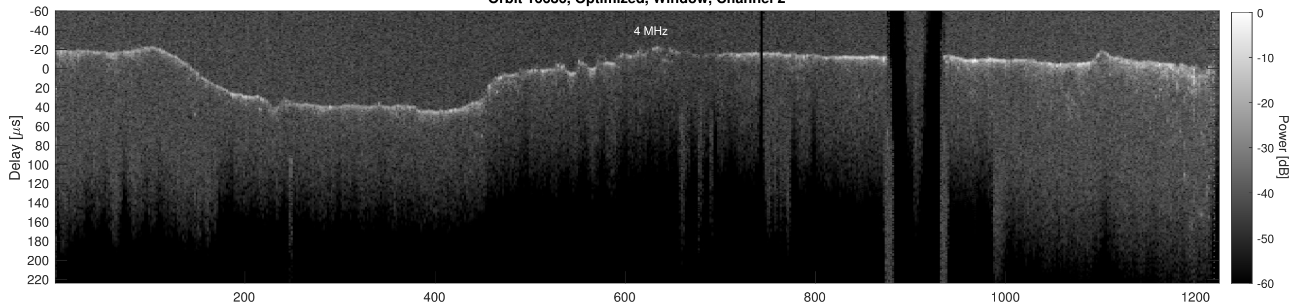
Orbit 16686, Cluttergram
