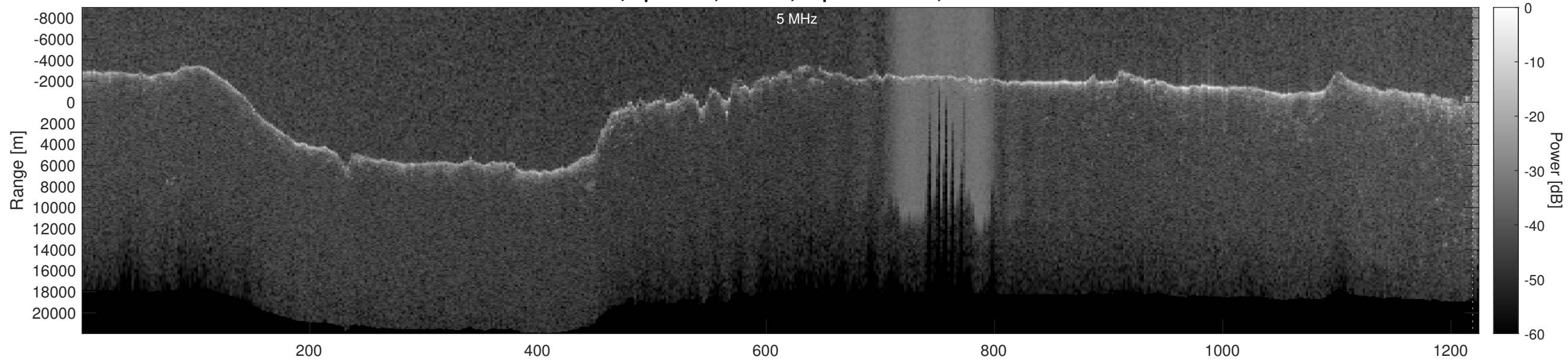
Orbit 16686, Optimized, Window, Depth-Corrected, Channel 2
