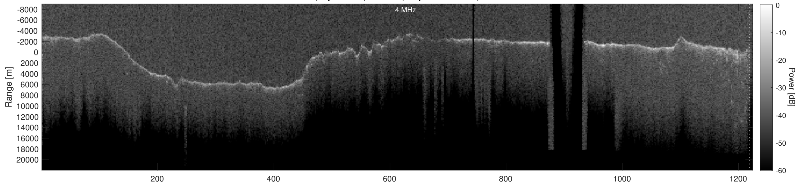
Orbit 16686, Depth-Corrected Cluttergram
