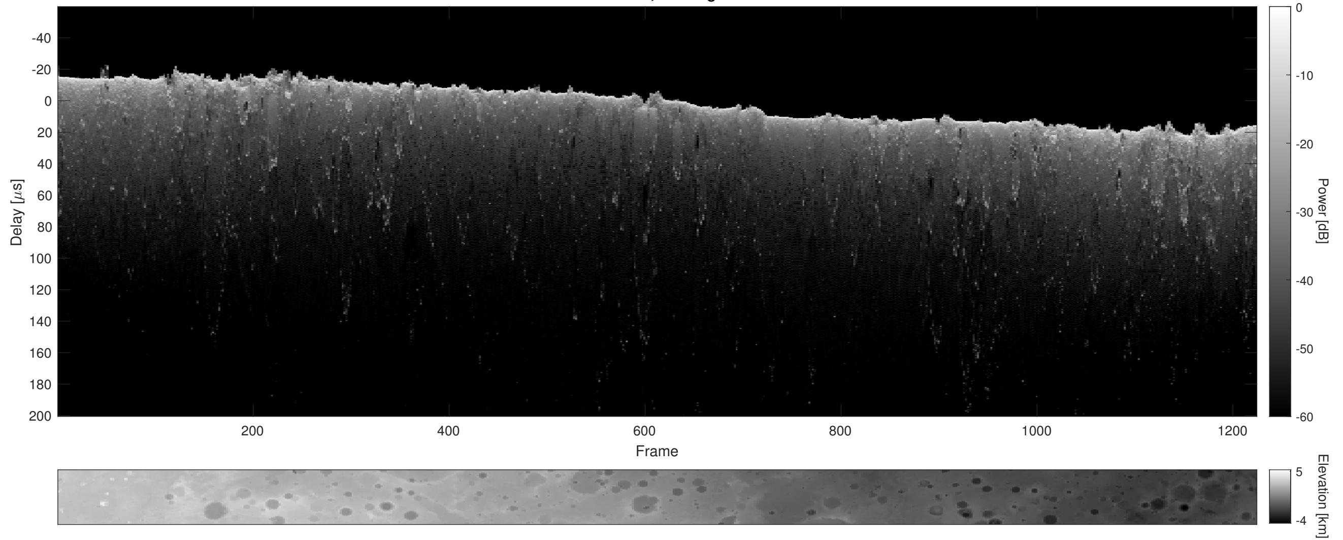
Orbit 16690, Cluttergram
