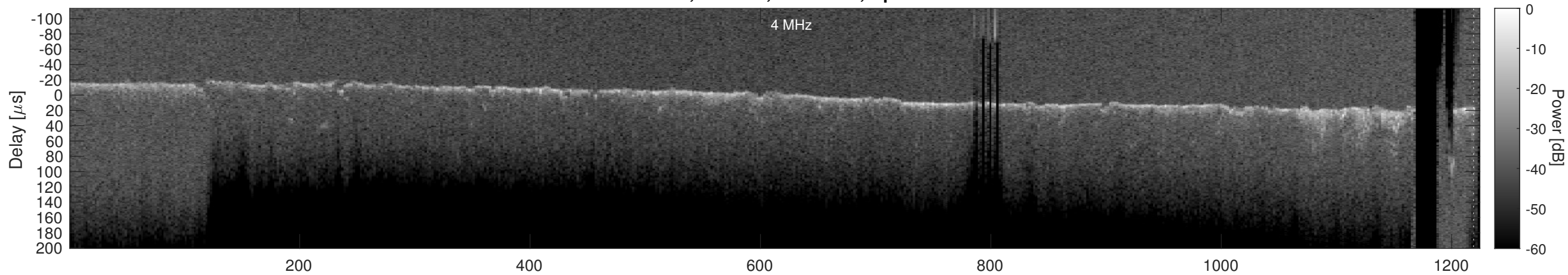
Orbit 16690, Cluttergram
