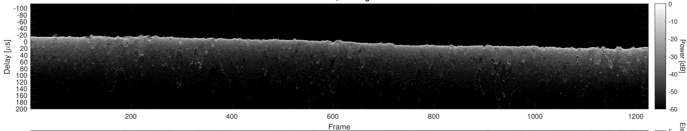
Orbit 16690, Cluttergram
