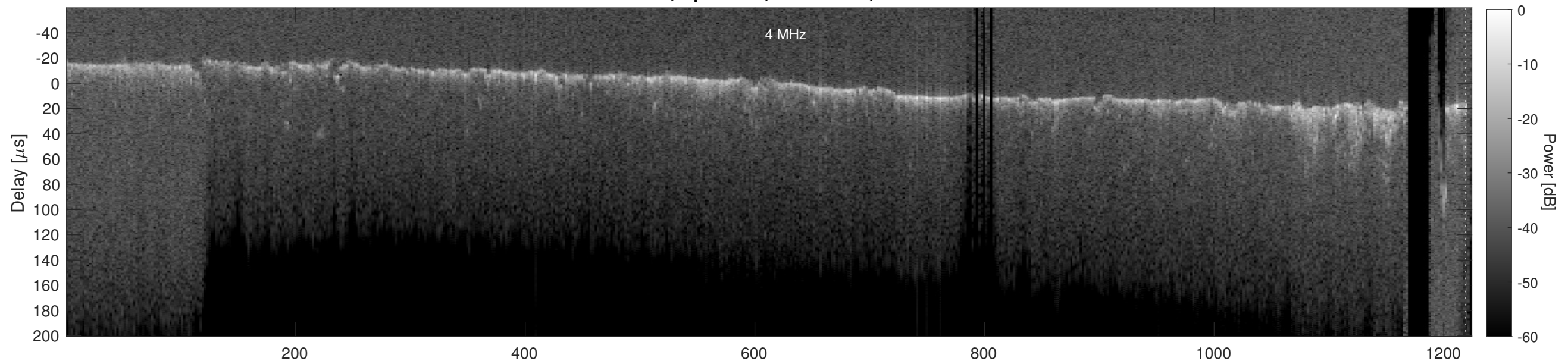
Orbit 16690, Cluttergram
