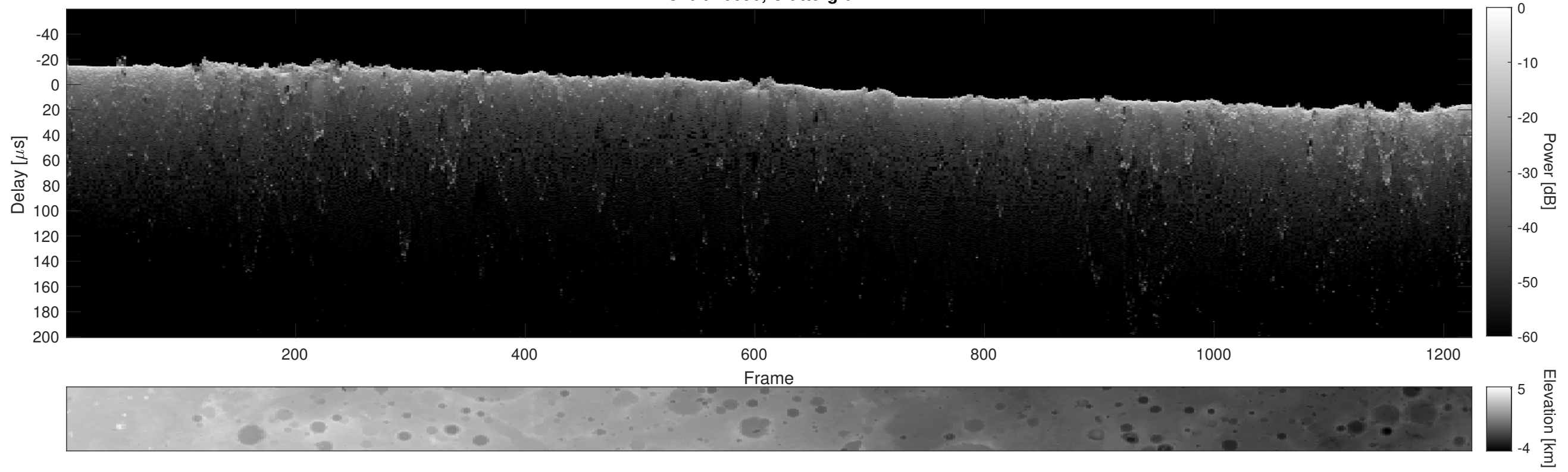
Orbit 16690, Cluttergram
