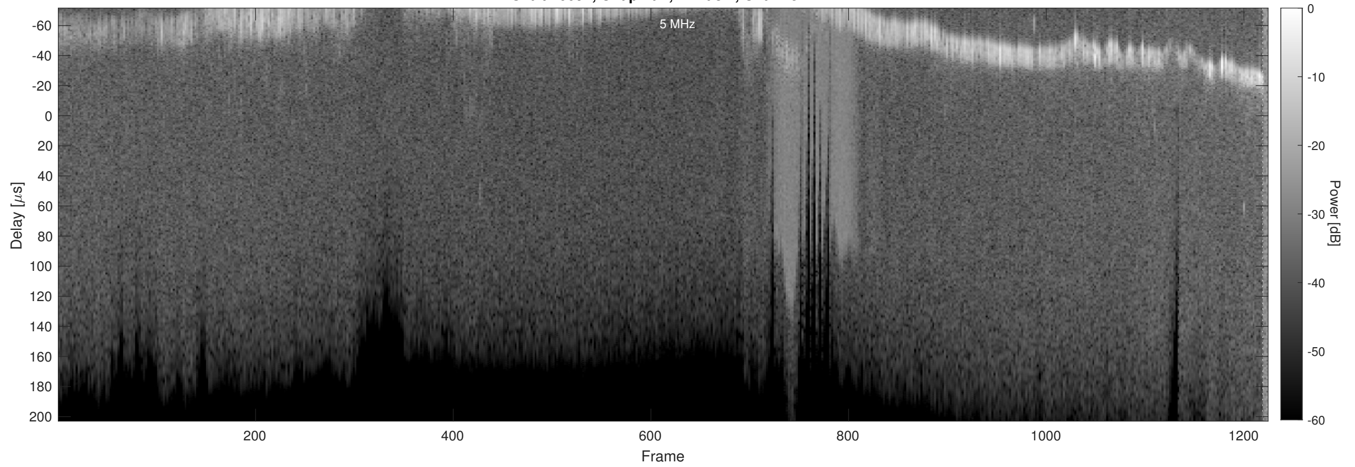
Orbit 16691, Chapman, Window, Channel 2
