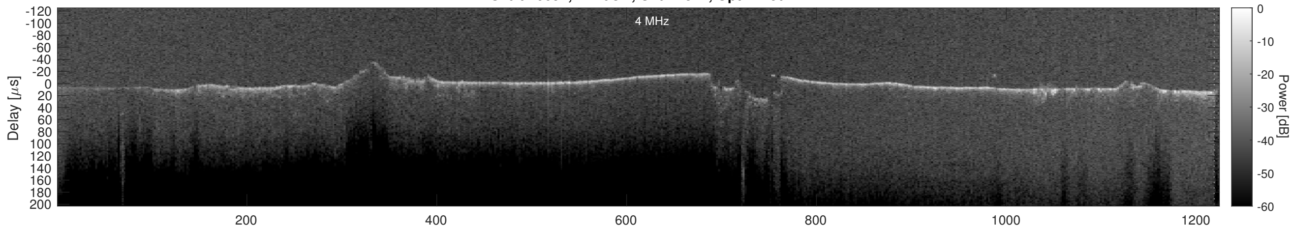
Orbit 16691, Cluttergram
