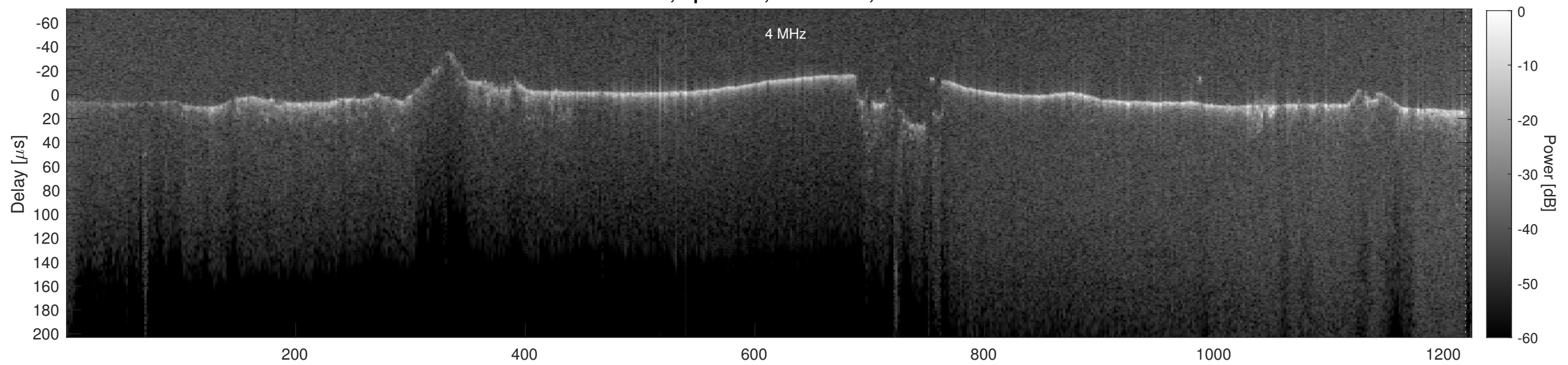
Orbit 16691, Cluttergram
