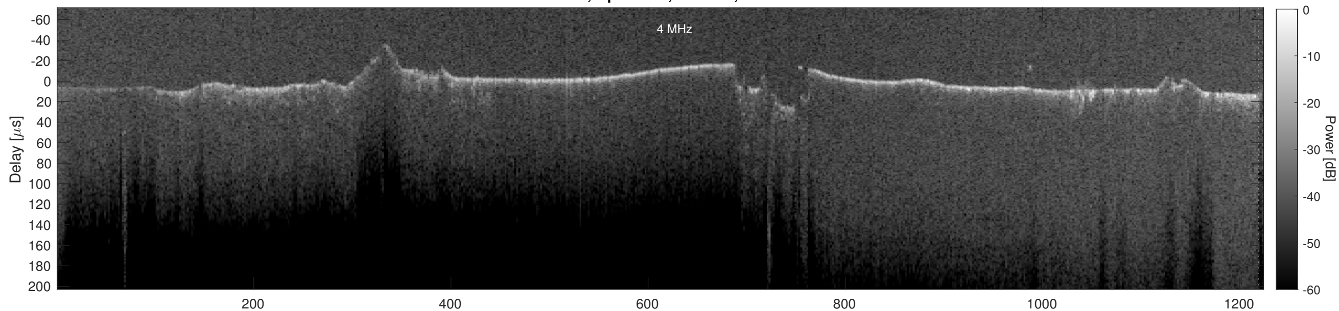
Orbit 16691, Cluttergram
