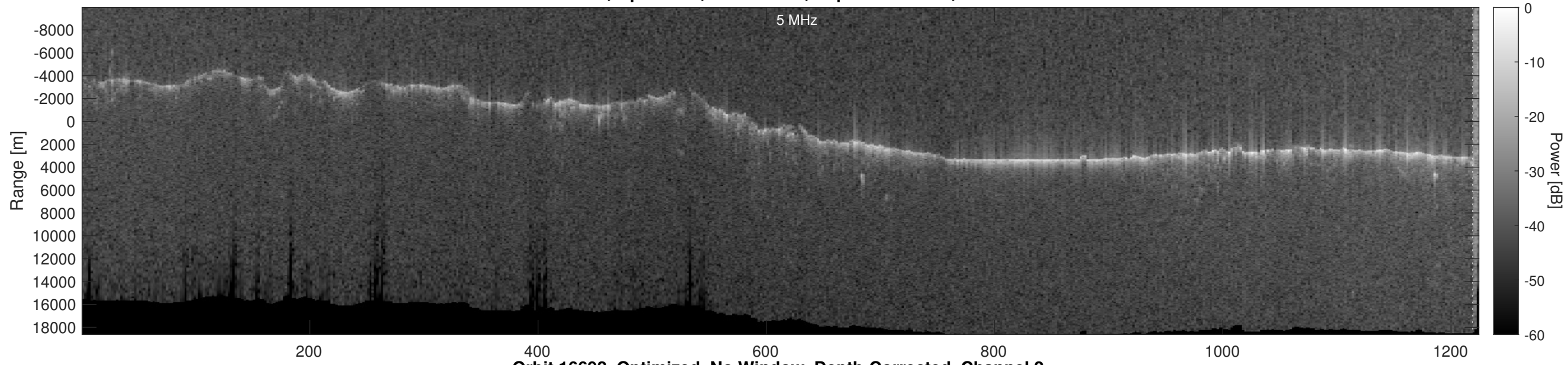
Orbit 16692, Optimized, No Window, Depth-Corrected, Channel 2
