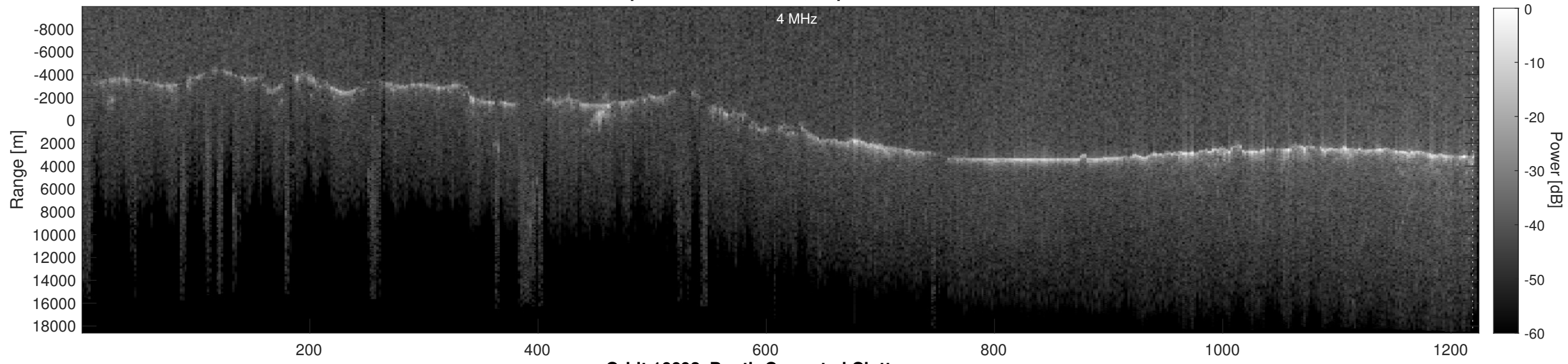
Orbit 16692, Depth-Corrected Cluttergram
