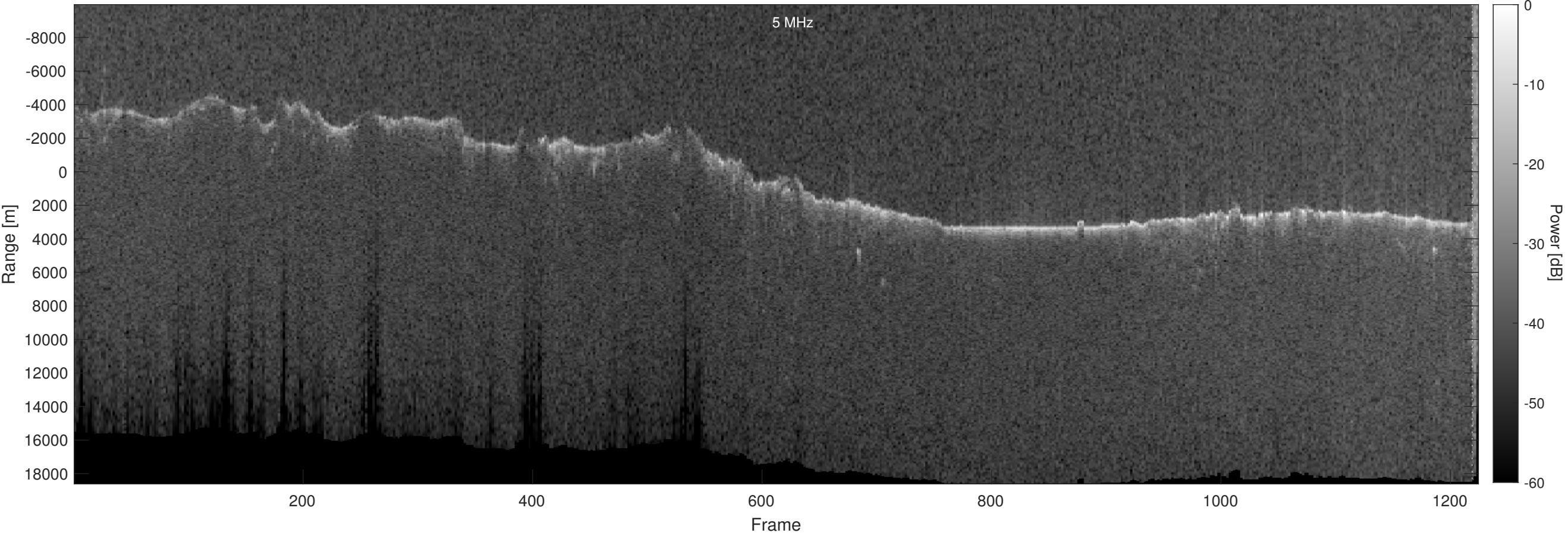
Orbit 16692, Optimized, Window, Depth-Corrected, Channel 2
