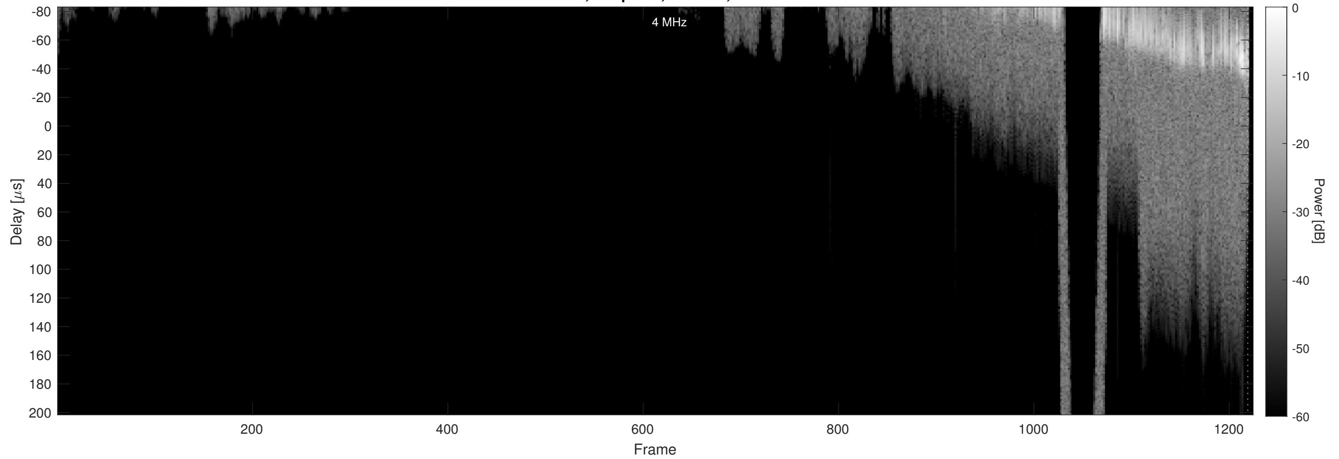
Orbit 16694, Chapman, Window, Channel 2
