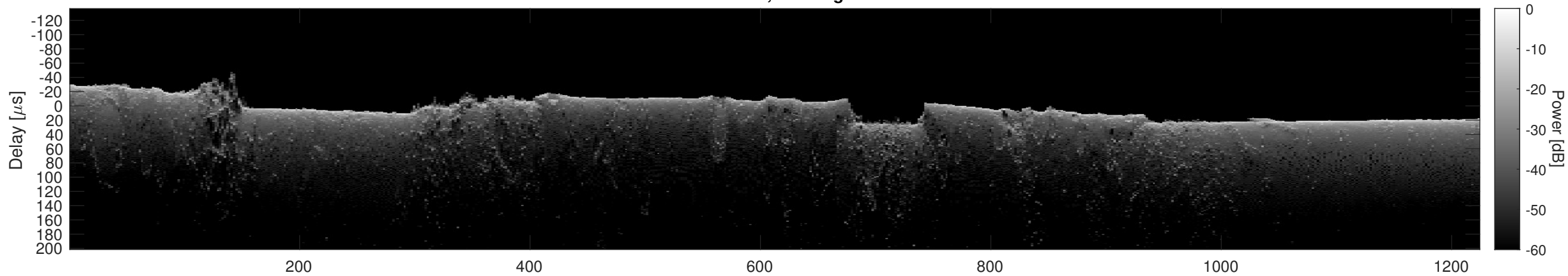
Orbit 16694, Cluttergram
