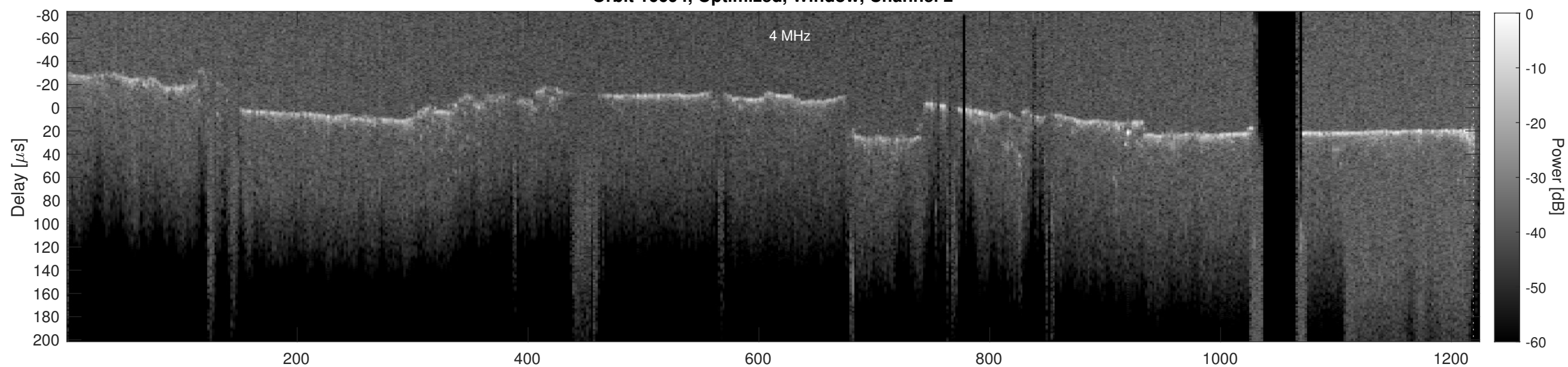
Orbit 16694, Cluttergram
