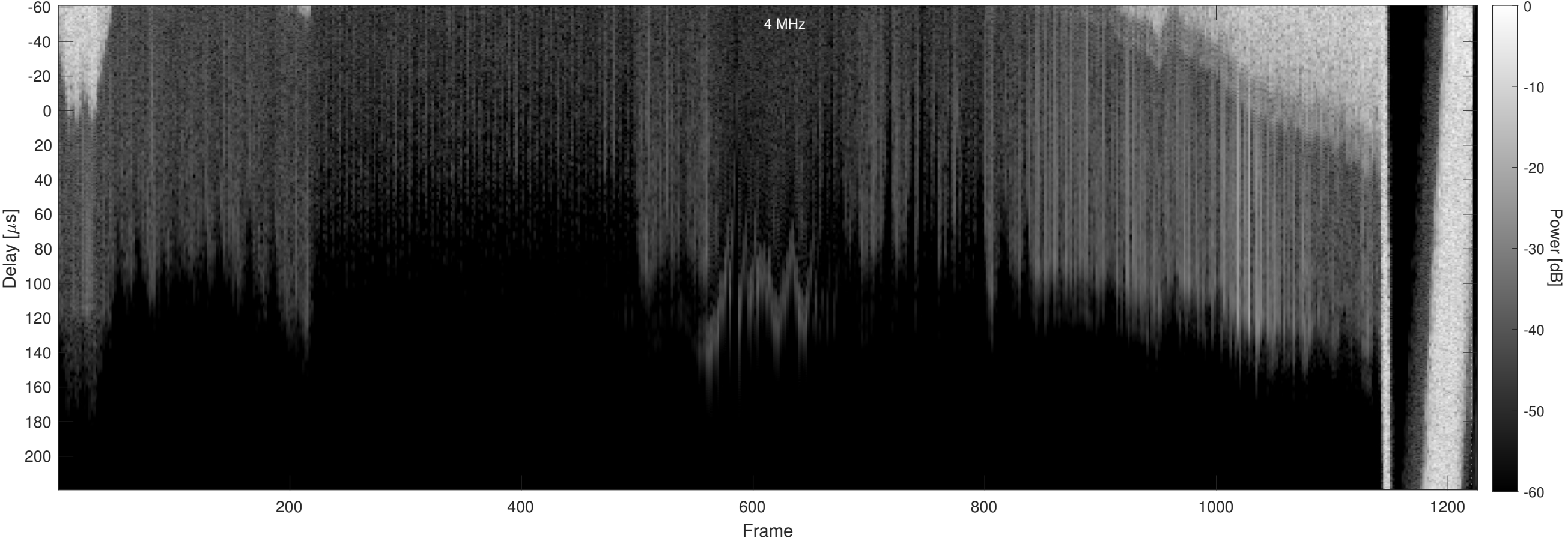
Orbit 16700, Chapman, No Window, Channel 2
