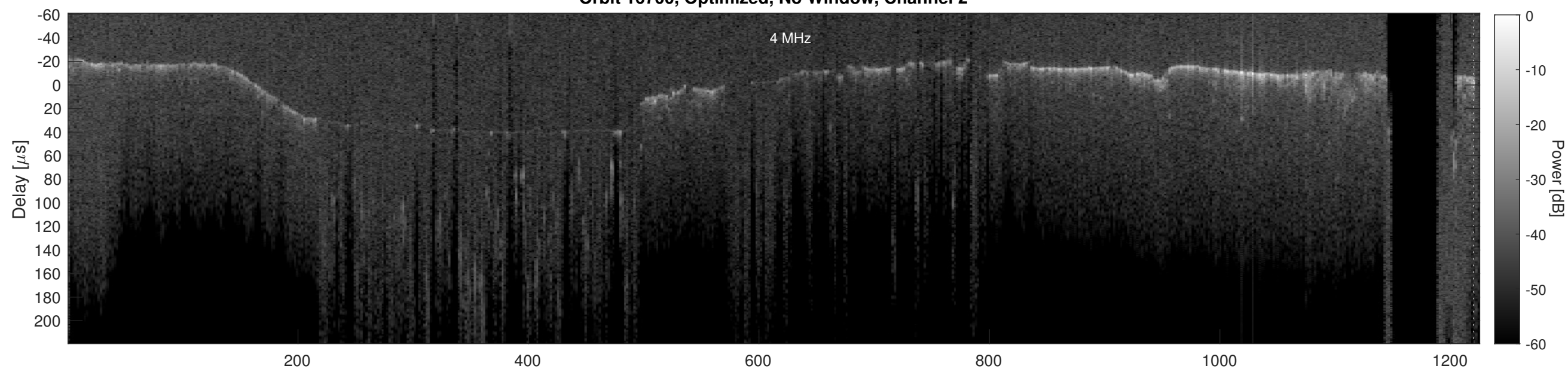
Orbit 16700, Cluttergram
