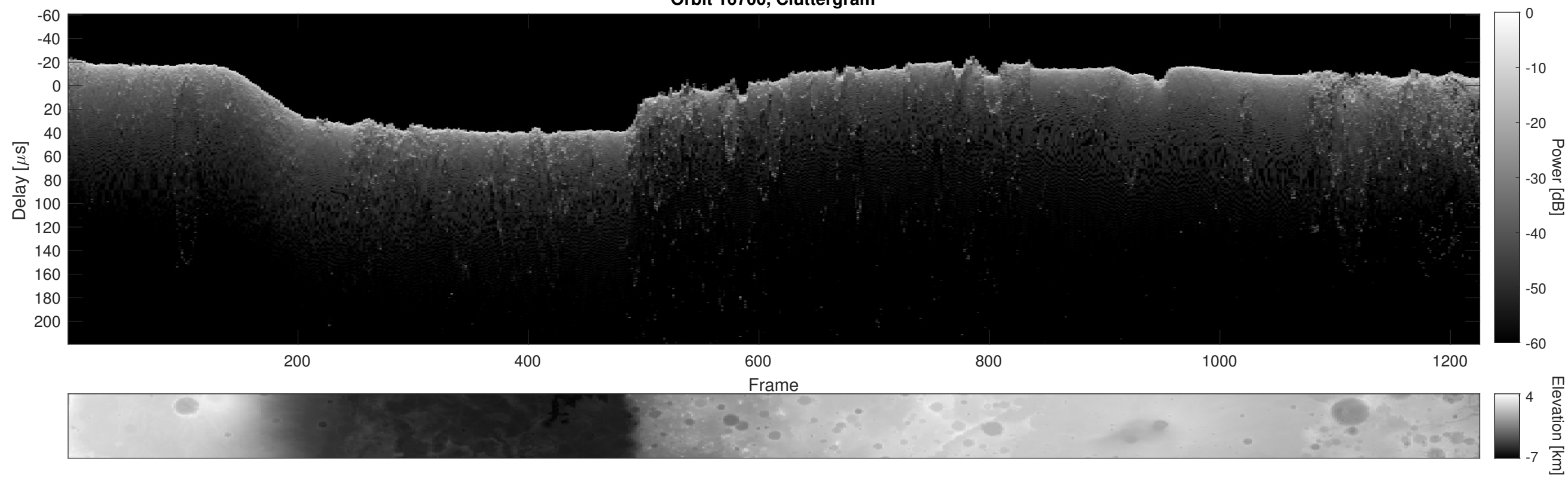
Orbit 16700, Cluttergram
