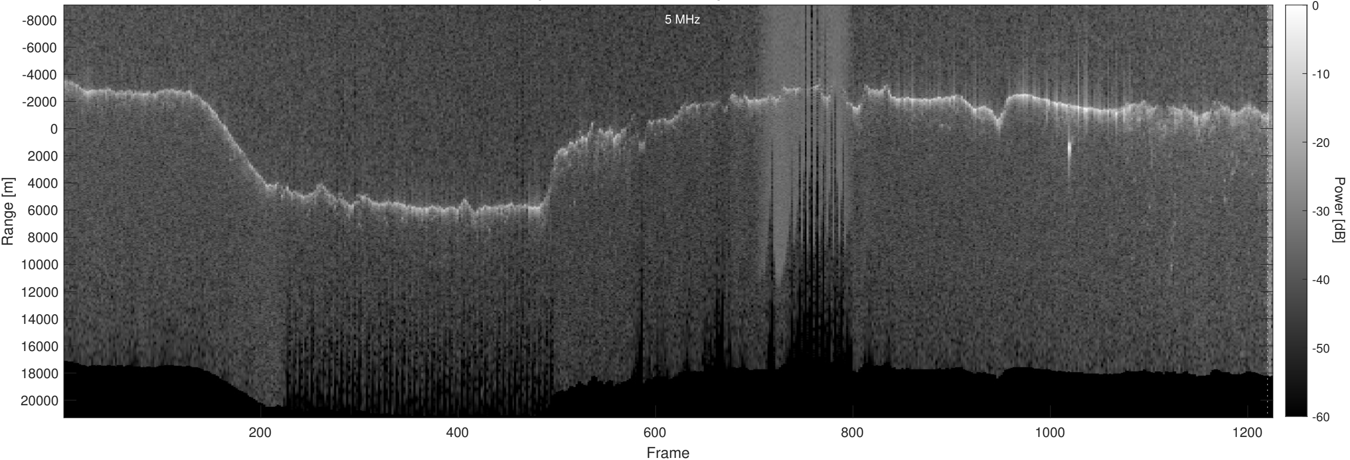
Orbit 16700, Optimized, No Window, Depth-Corrected, Channel 2
