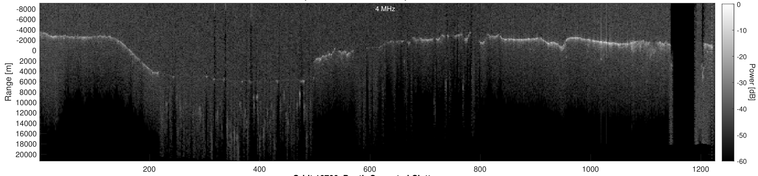
Orbit 16700, Depth-Corrected Cluttergram
