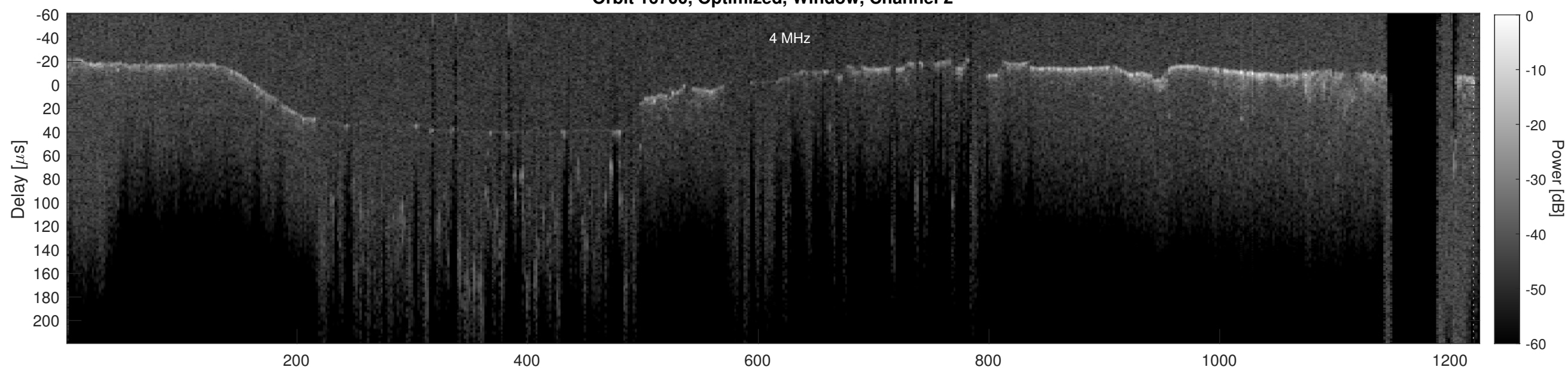
Orbit 16700, Cluttergram
