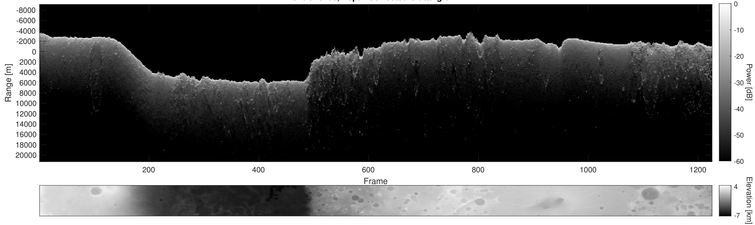
Orbit 16700, Depth-Corrected Cluttergram
