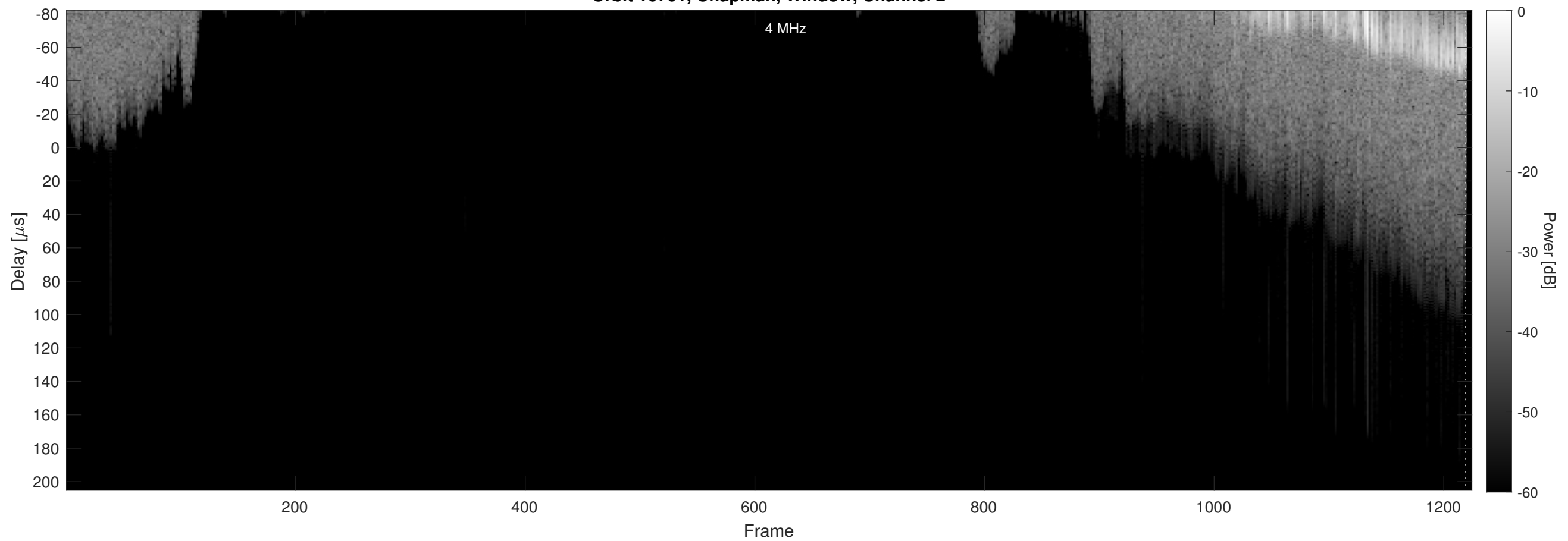
Orbit 16701, Chapman, Window, Channel 2
