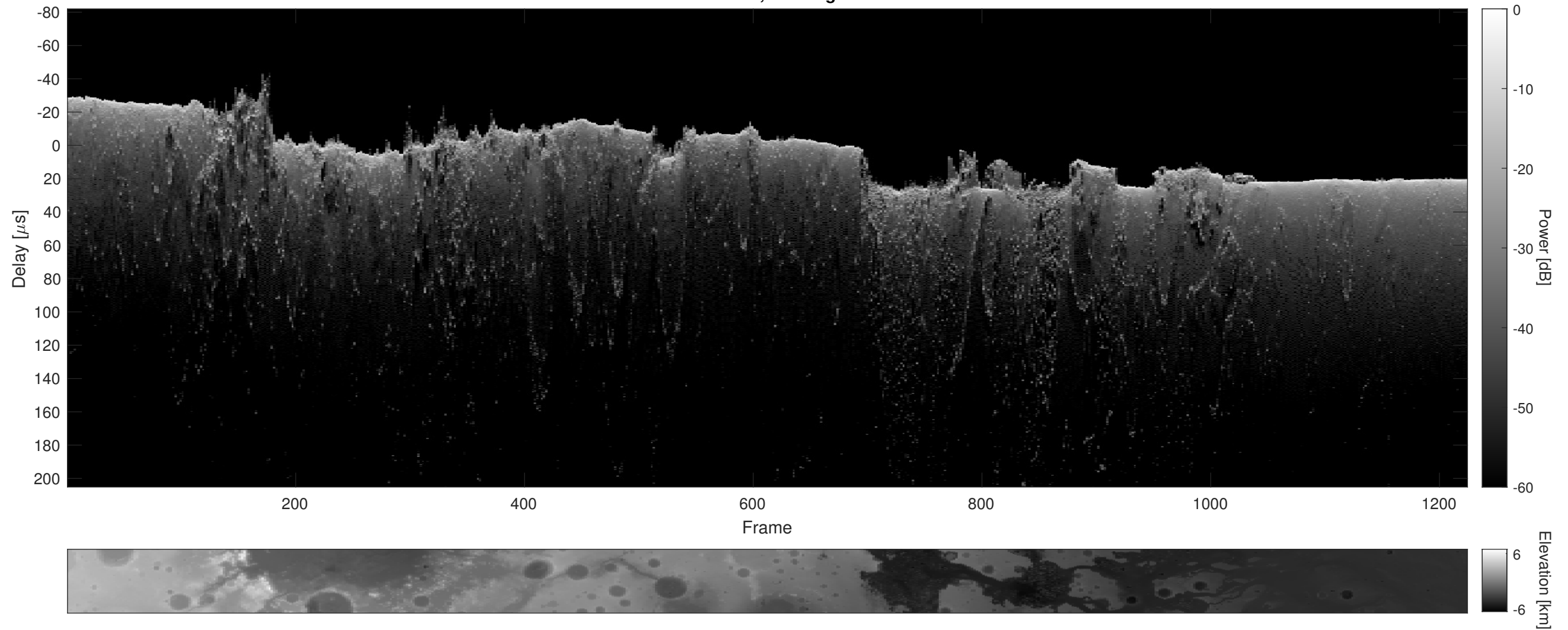
Orbit 16701, Cluttergram
