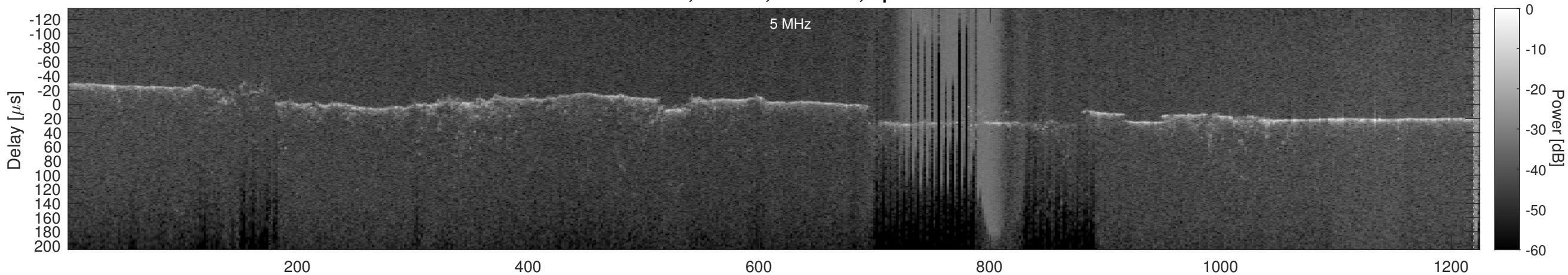
Orbit 16701, Cluttergram
