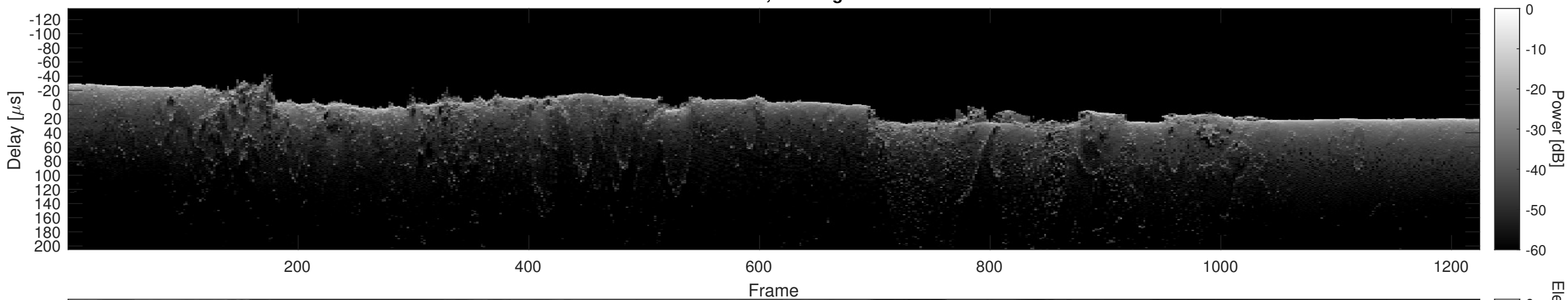
Orbit 16701, Cluttergram
