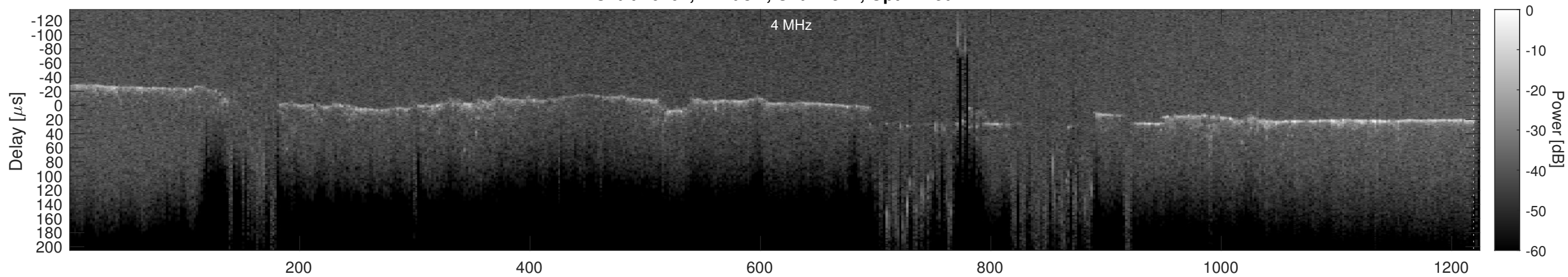
Orbit 16701, Cluttergram
