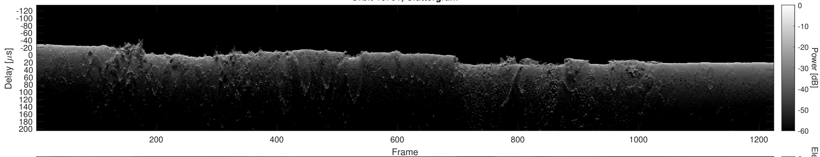
Orbit 16701, Cluttergram
