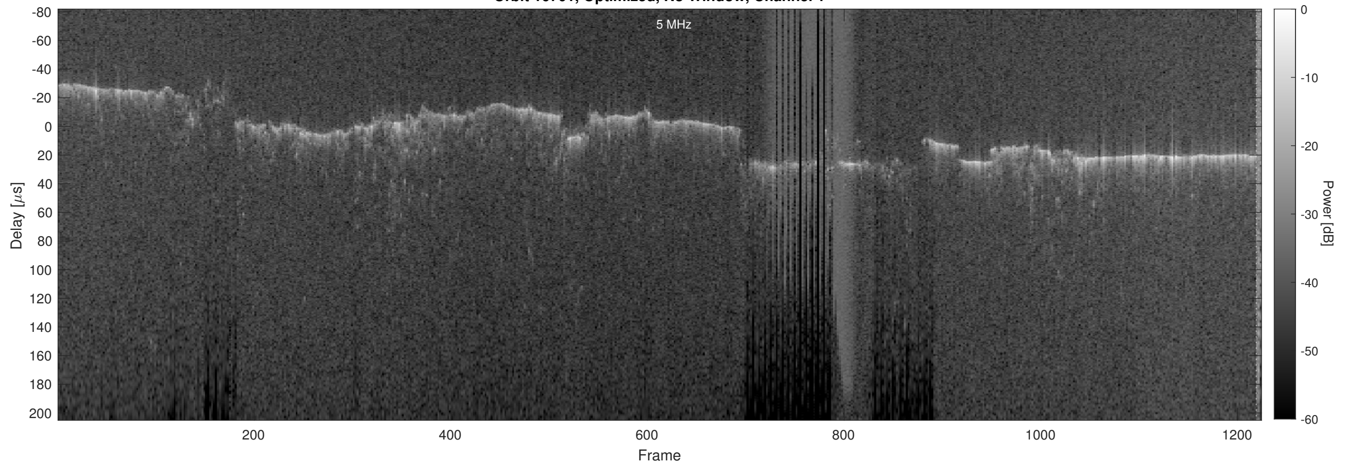
Orbit 16701, Optimized, No Window, Channel 2
