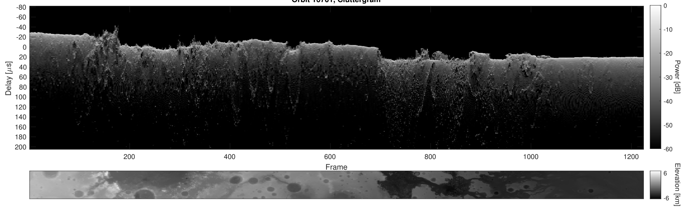
Orbit 16701, Cluttergram
