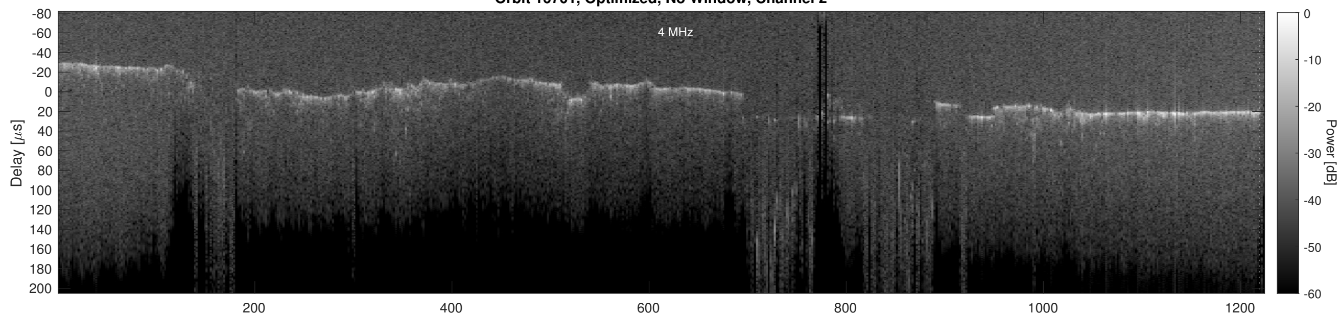
Orbit 16701, Cluttergram
