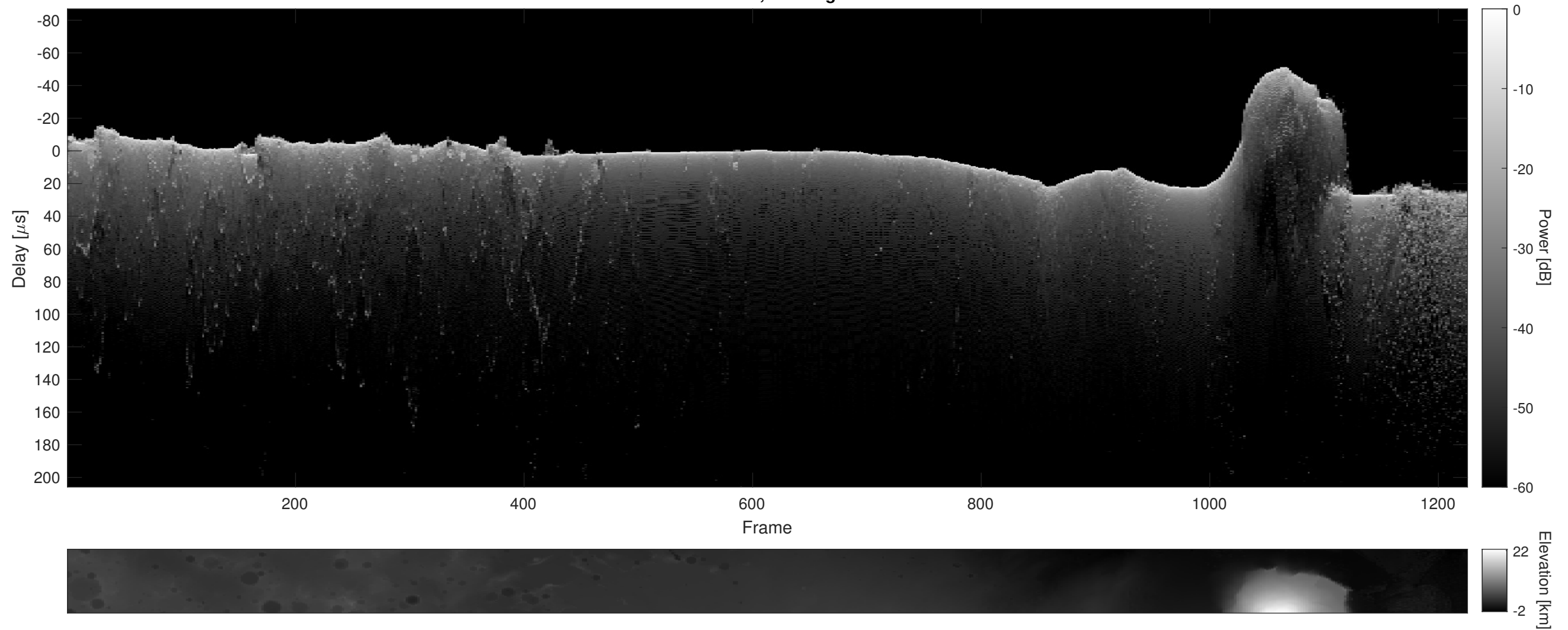
Orbit 16702, Cluttergram
