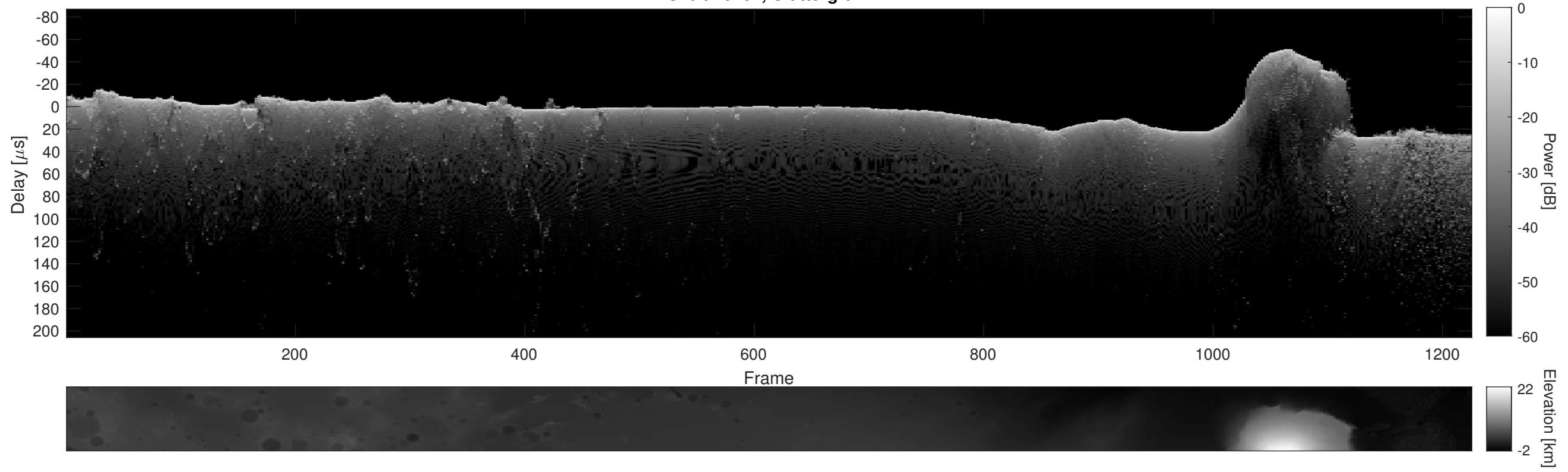
Orbit 16702, Cluttergram
