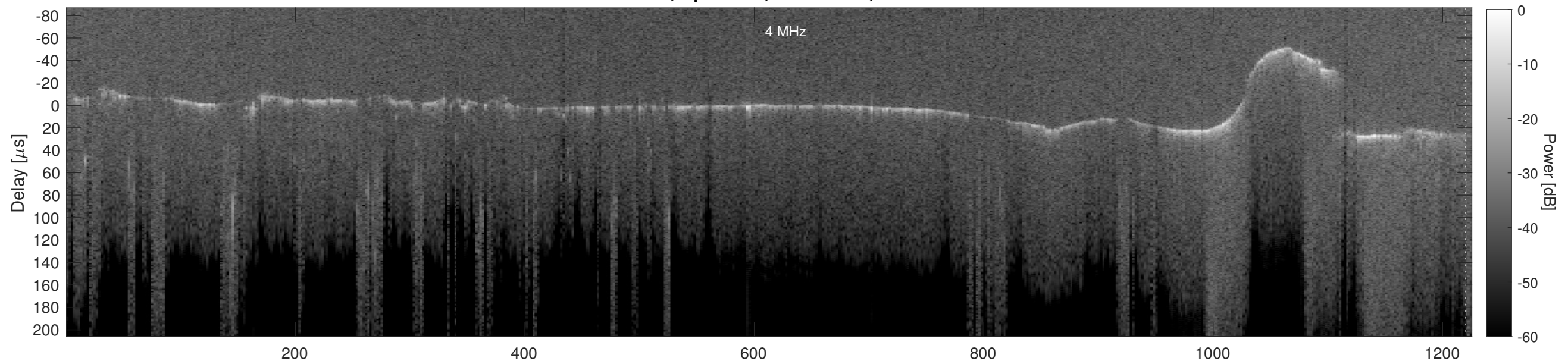
Orbit 16702, Cluttergram
